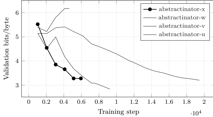
Figure 13: Bits per Byte across the 4 most recent experiments with comparable validation curves; the current experiment (abstractinator-x) is drawn in bold. Bold marks which run this build is reporting on , not which run scores best. The curves end wherever each run stopped, so they are at different points along their own training, and their endpoints are not a ranking. Generated from run logs - metrics that are not comparable across families (token loss vs. byte bits-per-byte vs. codec/CALM BrierLM) are excluded by construction, so the curves on this axis mean the same thing.
