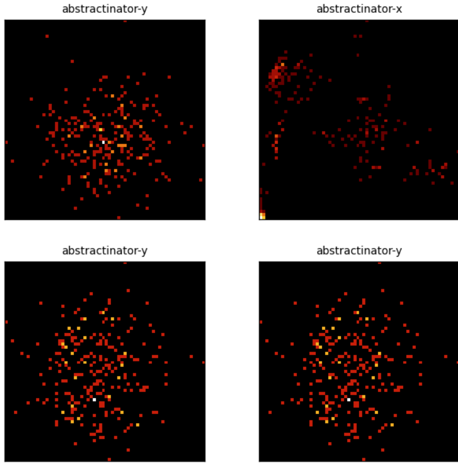
Figure 11: Center PCA density for the 4 most recent crystal-head runs (abstractinator-y, abstractinator-x, abstractinator-y, abstractinator-y). Each panel is the top-2 PCA projection of a head's vocabulary centers, binned to a 64 \times 64 density grid (log color) - the same snapshot the dashboard renders live. Different runs settle into structurally different geometries, not noise.
