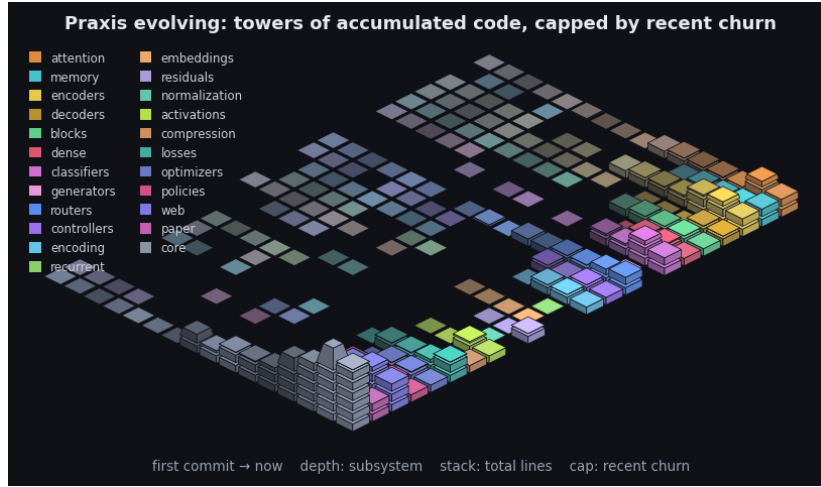
Figure 12: Praxis’s git history as an isometric terrain over the last 2619 commits. Each cell is one subsystem in one time window: a stack of base blocks for its accumulated size (total lines, recency-weighted) topped by a vivid cap for that window’s line churn - the standing codebase carrying the recent activity. Both are weighted by recency (the kernel the model applies to a sequence, turned on the repository): recent windows stack tall with bright caps while history thins toward the always-present prior - the low valley we roll into. Color fades from each subsystem’s hue toward a neutral prior into the past, banded in phased strata over a non-linear timescale. It is the bias/variance geometry read along the frequency axis (see the project notes): loud recent corrections over the quiet, ever-present base. By recency-weighted churn the current center of gravity is core, web, encoders. The framework charts the hand that builds it.
