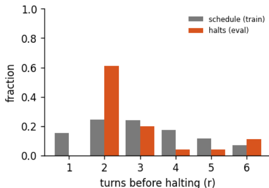
Figure 8: Halting distribution: the fraction of forward passes that stop after r turns, for the 6-turn recurrent loop of run abstractinator-g, early-halt rate 33%, mean boundary KL 0.29. schedule is the random loop-count the model trains under; halts is where the KL gate actually stops at inference. A mass pinned at the maximum (KL never collapsing) is the honest signature of a model that has not yet learned to converge early - the decision is real, not yet decisive.
