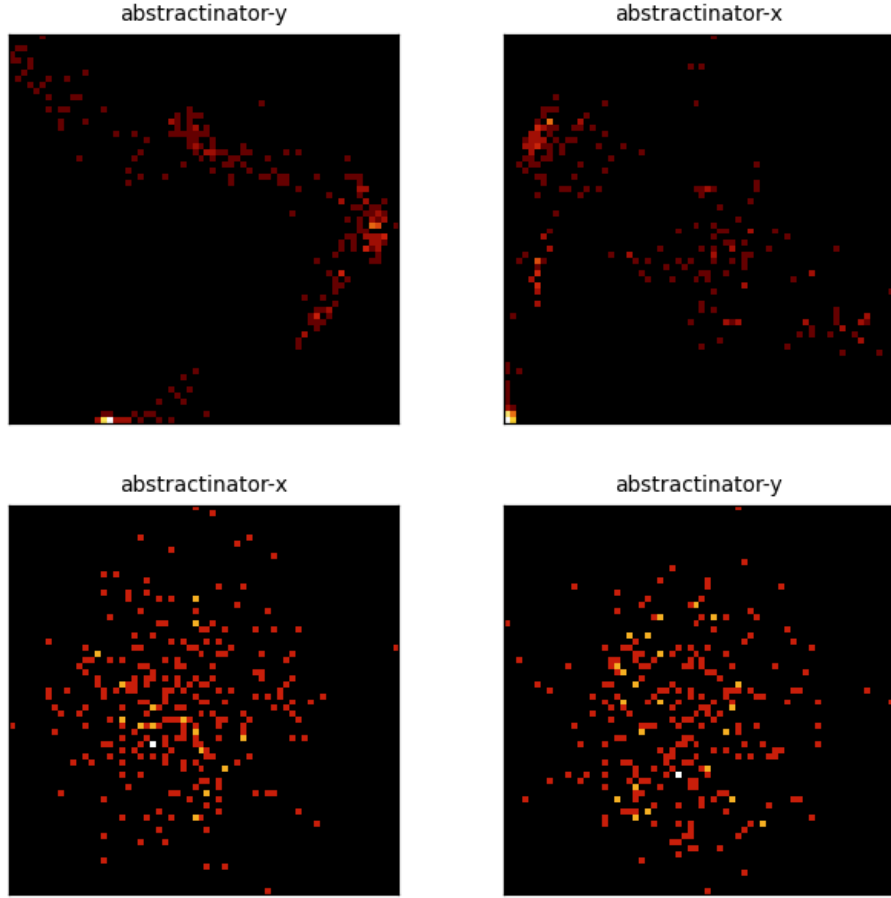
Figure 5: Center PCA density for the 4 most recent crystal-head runs (abstractinator-y, abstractinator-x, abstractinator-x, abstractinator-y). Each panel is the top-2 PCA projection of a head’s vocabulary centers, binned to a 64 \times 64 density grid (log color) - the same snapshot the dashboard renders live. Different runs settle into structurally different geometries, not noise.
