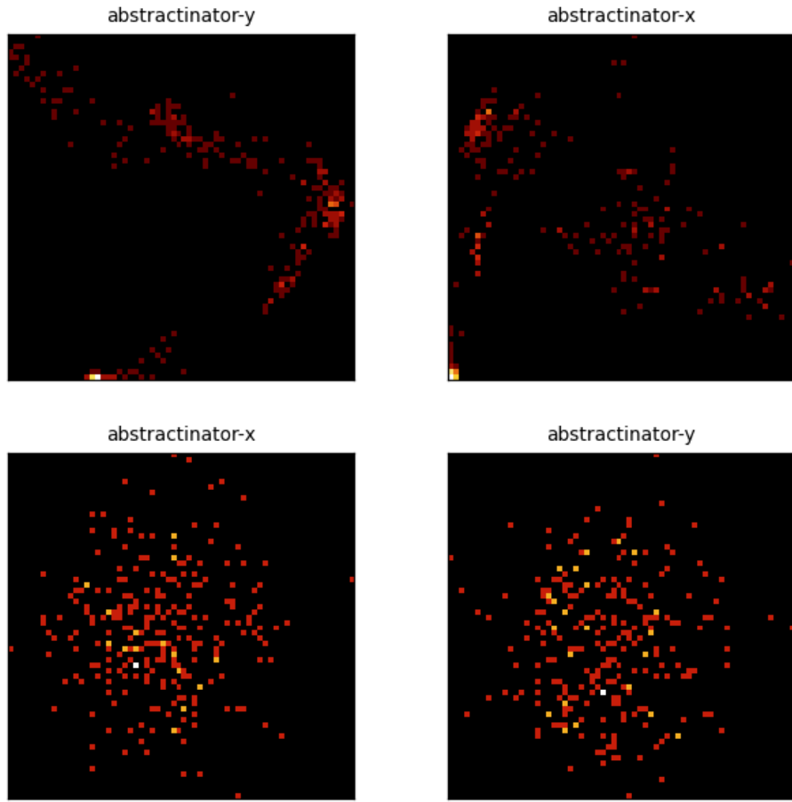
Figure 12: Center PCA density for the 4 most recent crystal-head runs (abstractinator-y, abstractinator-x, abstractinator-x, abstractinator-y). Each panel is the top-2 PCA projection of a head's vocabulary centers, binned to a 64 \times 64 density grid (log color) - the same snapshot the dashboard renders live. Different runs settle into structurally different geometries, not noise.
