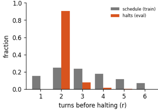
Figure 9: Halting distribution: the fraction of forward passes that stop after r turns, for the 6-turn recurrent loop of run abstractinator-y, early-halt rate 47%, mean boundary KL 1.01. schedule is the random loop-count the model trains under; halts is where the KL gate actually stops at inference. A mass pinned at the maximum (KL never collapsing) is the honest signature of a model that has not yet learned to converge early - the decision is real, not yet decisive.
