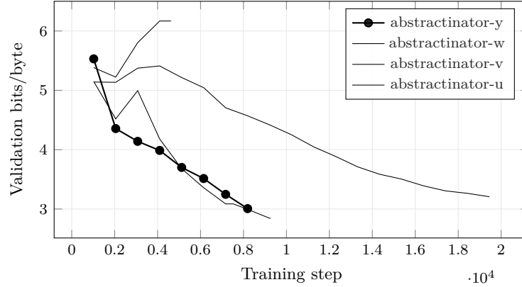
Figure 14: Bits per Byte across the 4 most recent experiments with comparable validation curves; the current experiment (abstractinator-y) is drawn in bold. Bold marks which run this build is reporting on , not which run scores best. The curves end wherever each run stopped, so they are at different points along their own training, and their endpoints are not a ranking. Generated from run logs - metrics that are not comparable across families (token loss vs. byte bits-per-byte vs. codec/CALM BrierLM) are excluded by construction, so the curves on this axis mean the same thing.
