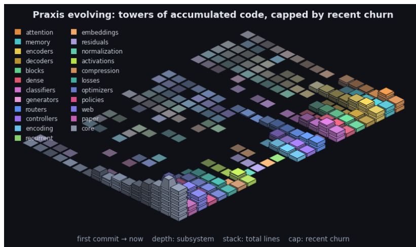
Figure 9: Praxis’s git history as an isometric terrain over the last 2675 commits. Each cell is one subsystem in one time window: a stack of base blocks for its accumulated size (total lines, recency-weighted) topped by a vivid cap for that window’s line churn - the standing codebase carrying the recent activity. Both are weighted by recency (the kernel the model applies to a sequence, turned on the repository): recent windows stack tall with bright caps while history thins toward the always-present prior - the low valley we roll into. Color fades from each subsystem’s hue toward a neutral prior into the past, banded in phased strata over a non-linear timescale. It is the bias/variance geometry read along the frequency axis (see the project notes): loud recent corrections over the quiet, ever-present base. By recency-weighted churn the current center of gravity is core, web, encoders. The framework charts the hand that builds it.
