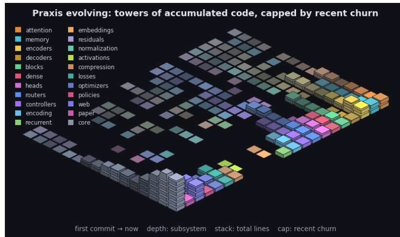
Figure 7: Praxis’s git history as an isometric terrain over the last 2230 commits. Each cell is one subsystem in one time window: a stack of base blocks for its accumulated size (total lines, recency-weighted) topped by a vivid cap for that window’s line churn - the standing codebase carrying the recent activity. Both are weighted by recency (the kernel the model applies to a sequence, turned on the repository): recent windows stack tall with bright caps while history thins toward the always-present prior - the low valley we roll into. Color fades from each subsystem’s hue toward a neutral prior into the past, banded in phased strata over a non-linear timescale. It is the bias/variance geometry read along the frequency axis (see the project notes): loud recent corrections over the quiet, ever-present base. By recency-weighted churn the current center of gravity is core, web, encoders. The framework charts the hand that builds it.
