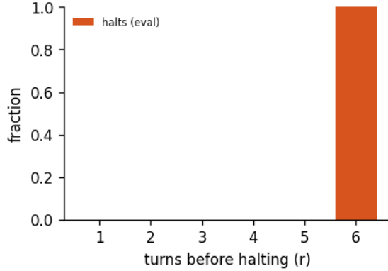
Figure 5: Halting distribution: the fraction of forward passes that stop after r turns, for the 6-turn recurrent loop of run calm-d, early-halt rate 0%, mean boundary KL 3.24. schedule is the random loop-count the model trains under; halts is where the KL gate actually stops at inference. A mass pinned at the maximum (KL never collapsing) is the honest signature of a model that has not yet learned to converge early - the decision is real, not yet decisive.
