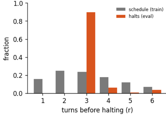
Figure 8: Halting distribution: the fraction of forward passes that stop after r turns, for the 6-turn recurrent loop of run abstractinator-v, early-halt rate 31%, mean boundary KL 0.61. schedule is the random loop-count the model trains under; halts is where the KL gate actually stops at inference. A mass pinned at the maximum (KL never collapsing) is the honest signature of a model that has not yet learned to converge early - the decision is real, not yet decisive.
