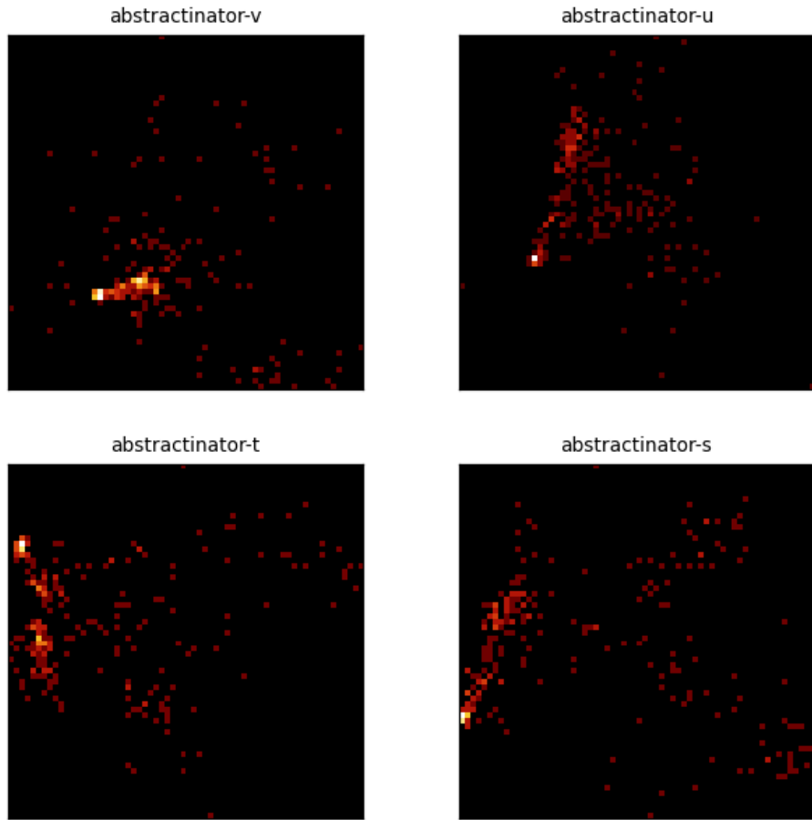
Figure 11: Center PCA density for the 4 most recent crystal-head runs (abstractinator-v, abstractinator-u, abstractinator-t, abstractinator-s). Each panel is the top-2 PCA projection of a head's vocabulary centers, binned to a 64 \times 64 density grid (log color) - the same snapshot the dashboard renders live. Different runs settle into structurally different geometries, not noise.
