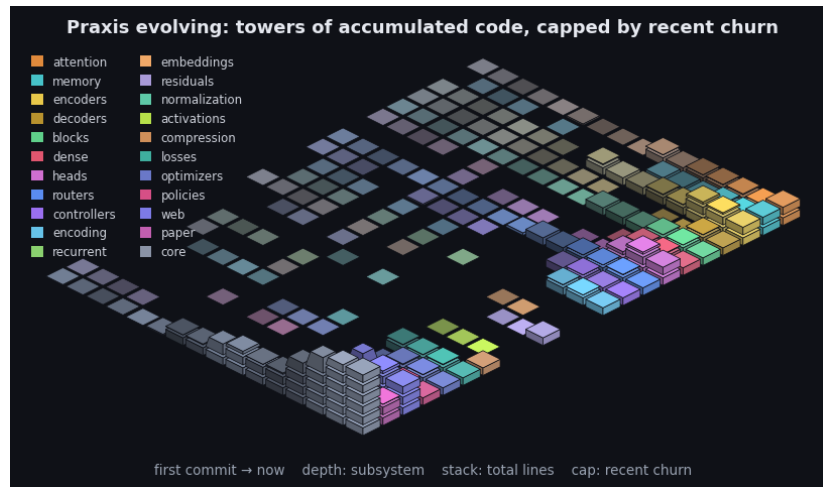
Figure 12: Praxis’s git history as an isometric terrain over the last 2458 commits. Each cell is one subsystem in one time window: a stack of base blocks for its accumulated size (total lines, recency-weighted) topped by a vivid cap for that window’s line churn - the standing codebase carrying the recent activity. Both are weighted by recency (the kernel the model applies to a sequence, turned on the repository): recent windows stack tall with bright caps while history thins toward the always-present prior - the low valley we roll into. Color fades from each subsystem’s hue toward a neutral prior into the past, banded in phased strata over a non-linear timescale. It is the bias/variance geometry read along the frequency axis (see the project notes): loud recent corrections over the quiet, ever-present base. By recency-weighted churn the current center of gravity is core, web, paper. The framework charts the hand that builds it.
