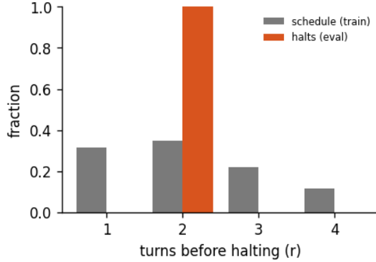
Figure 8: Halting distribution: the fraction of forward passes that stop after r turns, for the 4-turn recurrent loop of run abstractinator-g, early-halt rate 50%, mean boundary KL 0.217. schedule is the random loop-count the model trains under; halts is where the KL gate actually stops at inference. A mass pinned at the maximum (KL never collapsing) is the honest signature of a model that has not yet learned to converge early - the decision is real, not yet decisive.
