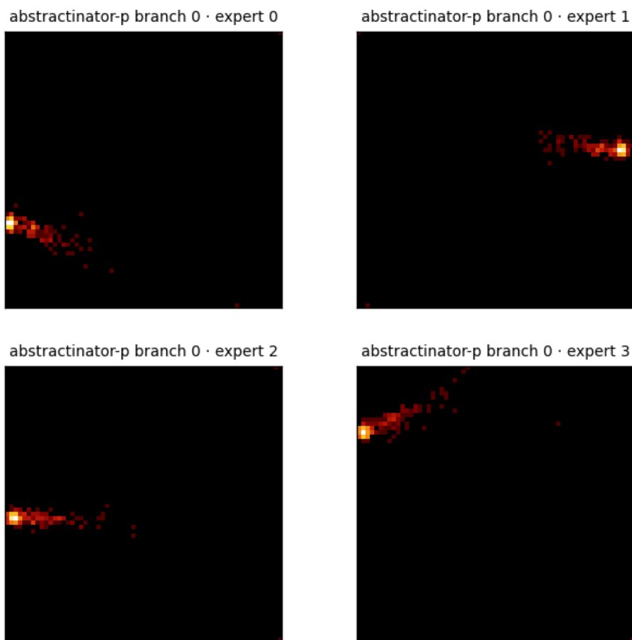
Figure 11: Center PCA density for the 4 crystal heads of abstractinator-p - a single multi-head model (prismatic6’s VEAR crystal bank), so these are that run’s own heads (branch 0 · expert 0, branch 0 · expert 1, branch 0 · expert 2, branch 0 · expert 3), not a cross-run mix. Each panel is the top-2 PCA projection of a head’s vocabulary centers, binned to a 64 \times 64 density grid (log color) - the same snapshot the dashboard renders live. The bank’s experts settle into structurally distinct geometries - the between-expert variance the router selects over.
