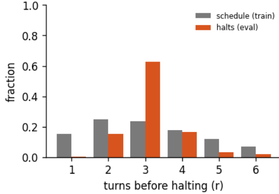
Figure 8: Halting distribution: the fraction of forward passes that stop after r turns, for the 6-turn recurrent loop of run abstractinator-p, early-halt rate 32%, mean boundary KL 0.195. schedule is the random loop-count the model trains under; halts is where the KL gate actually stops at inference. A mass pinned at the maximum (KL never collapsing) is the honest signature of a model that has not yet learned to converge early - the decision is real, not yet decisive.
