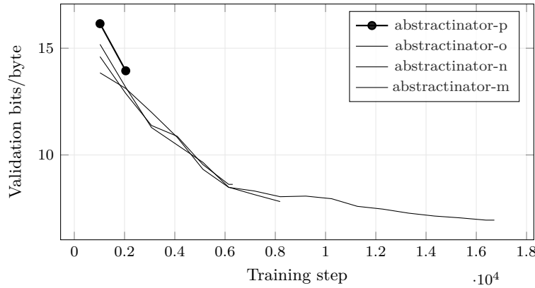
Figure 13: Bits per Byte across the 4 most recent experiments with comparable validation curves; the current experiment ( abstractinator-p ) is drawn in bold. Bold marks which run this build is reporting on , not which run scores best. The curves end wherever each run stopped, so they are at different points along their own training, and their endpoints are not a ranking. Generated from run logs - metrics that are not comparable across families (token loss vs. byte bits-per-byte vs. codec/CALM BrierLM) are excluded by construction, so the curves on this axis mean the same thing.
