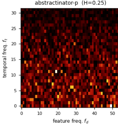
Figure 2: The static amplitude spectrum |a[f_t, f_d]| for abstractinator-p - the learned grid that, inverse-transformed through the frozen Weyl phases, becomes the bias field. This is the heatmap the text describes: energy that settles into a low-frequency band (small f_t, f_d ) is the corpus rhythm crystallizing, while a grid that stays uniform is a field still indistinguishable from noise. Hoyer concentration H = 0.25 quantifies it on the same [0, 1] scale the prose names (1 = a single cell, 0 = uniform), computed from this very tensor by concentration() - the same value the dashboard logs live. The pink 1/f^\alpha prior lives in the frozen basis, not in these amplitudes, so the grid shown is exactly what the head exposes.
