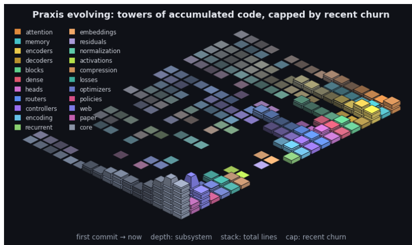
Figure 4: Praxis’s git history as an isometric terrain over the last 2319 commits. Each cell is one subsystem in one time window: a stack of base blocks for its accumulated size (total lines, recency-weighted) topped by a vivid cap for that window’s line churn - the standing codebase carrying the recent activity. Both are weighted by recency (the kernel the model applies to a sequence, turned on the repository): recent windows stack tall with bright caps while history thins toward the always-present prior - the low valley we roll into. Color fades from each subsystem’s hue toward a neutral prior into the past, banded in phased strata over a non-linear timescale. It is the bias/variance geometry read along the frequency axis (see the project notes): loud recent corrections over the quiet, ever-present base. By recency-weighted churn the current center of gravity is core, web, paper. The framework charts the hand that builds it.
