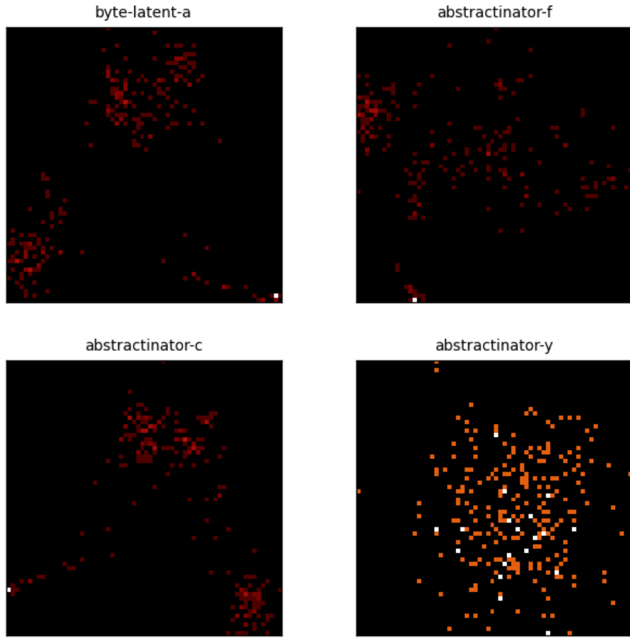
Figure 12: Center PCA density for the 4 most recent crystal-head runs ( byte-latent-a , abstractinator-f , abstractinator-c , abstractinator-y ). Each panel is the top-2 PCA projection of a head’s vocabulary centers, binned to a 64 \times 64 density grid (log color) - the same snapshot the dashboard renders live. Different runs settle into structurally different geometries, not noise.
