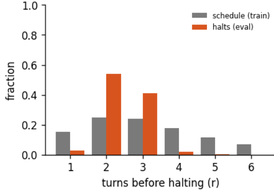
Figure 9: Halting distribution: the fraction of forward passes that stop after r turns, for the 6-turn recurrent loop of run byte-latent-a, early-halt rate 41%, mean boundary KL 0.018. schedule is the random loop-count the model trains under; halts is where the KL gate actually stops at inference. A mass pinned at the maximum (KL never collapsing) is the honest signature of a model that has not yet learned to converge early - the decision is real, not yet decisive.
