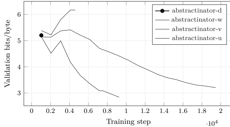
Figure 10: Bits per Byte across the 4 most recent experiments with comparable validation curves; the current experiment (abstractinator-d) is drawn in bold. Bold marks which run this build is reporting on , not which run scores best. The curves end wherever each run stopped, so they are at different points along their own training, and their endpoints are not a ranking. Generated from run logs - metrics that are not comparable across families (token loss vs. byte bits-per-byte vs. codec/CALM BrierLM) are excluded by construction, so the curves on this axis mean the same thing.
