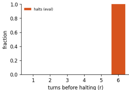
Figure 3: Halting distribution: the fraction of forward passes that stop after r turns, for the 6-turn recurrent loop of run calm-f, early-halt rate 0%, mean boundary KL 2.58. schedule is the random loop-count the model trains under; halts is where the KL gate actually stops at inference. A mass pinned at the maximum (KL never collapsing) is the honest signature of a model that has not yet learned to converge early - the decision is real, not yet decisive.
