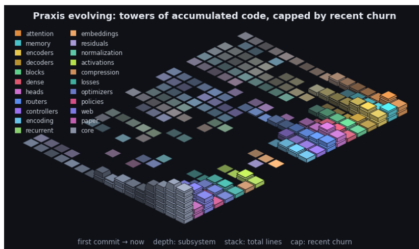
Figure 13: Praxis’s git history as an isometric terrain over the last 2591 commits. Each cell is one subsystem in one time window: a stack of base blocks for its accumulated size (total lines, recency-weighted) topped by a vivid cap for that window’s line churn - the standing codebase carrying the recent activity. Both are weighted by recency (the kernel the model applies to a sequence, turned on the repository): recent windows stack tall with bright caps while history thins toward the always-present prior - the low valley we roll into. Color fades from each subsystem’s hue toward a neutral prior into the past, banded in phased strata over a non-linear timescale. It is the bias/variance geometry read along the frequency axis (see the project notes): loud recent corrections over the quiet, ever-present base. By recency-weighted churn the current center of gravity is core, web, paper. The framework charts the hand that builds it.
