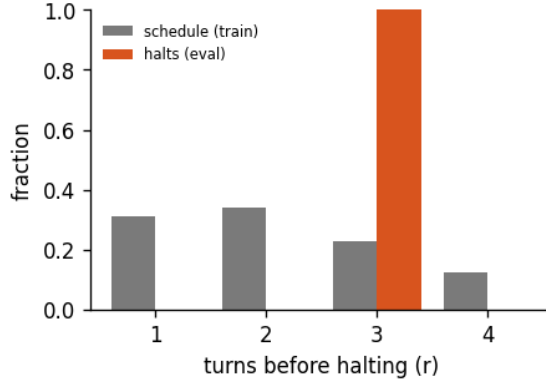
Figure 2: Halting distribution: the fraction of forward passes that stop after r turns, for the 4-turn recurrent loop of run calm-d-1, early-halt rate 33%, mean boundary KL 0.206. schedule is the random loop-count the model trains under; halts is where the KL gate actually stops at inference. A mass pinned at the maximum (KL never collapsing) is the honest signature of a model that has not yet learned to converge early - the decision is real, not yet decisive.
