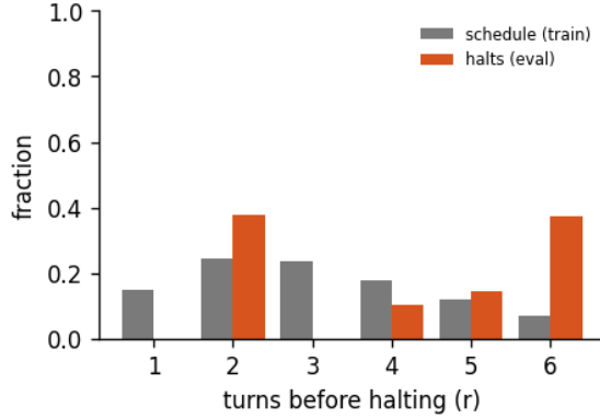
Figure 8: Halting distribution: the fraction of forward passes that stop after r turns, for the 6-turn recurrent loop of run abstractinator-m, early-halt rate 17%, mean boundary KL 0.411. schedule is the random loop-count the model trains under; halts is where the KL gate actually stops at inference. A mass pinned at the maximum (KL never collapsing) is the honest signature of a model that has not yet learned to converge early - the decision is real, not yet decisive.
