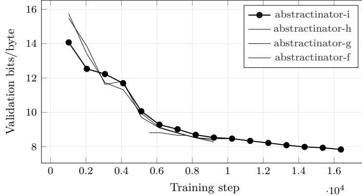
Figure 13: Bits per Byte across the 4 most recent experiments with comparable validation curves; the current experiment (abstractinator-i) is drawn in bold. Bold marks which run this build is reporting on , not which run scores best. The curves end wherever each run stopped, so they are at different points along their own training, and their endpoints are not a ranking. Generated from run logs - metrics that are not comparable across families (token loss vs. byte bits-per-byte vs. codec/CALM BrierLM) are excluded by construction, so the curves on this axis mean the same thing.
