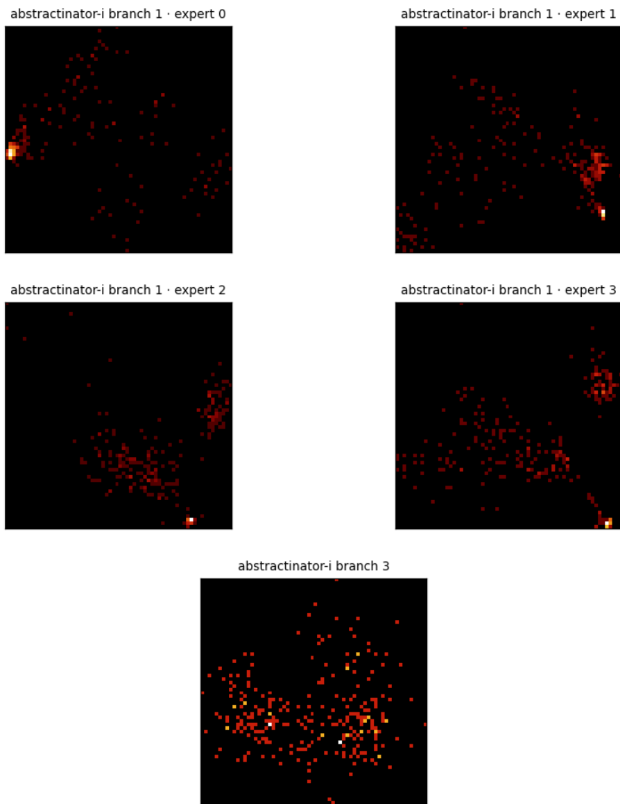
Figure 11: Center PCA density for the 5 crystal heads of abstractinator-i - a single multi-head model (prismatic4’s VEAR crystal bank), so these are that run’s own heads (branch 1 · expert 0, branch 1 · expert 1, branch 1 · expert 2, branch 1 · expert 3, branch 3), not a cross-run mix. Each panel is the top-2 PCA projection of a head’s vocabulary centers, binned to a 64 \times 64 density grid (log color) - the same snapshot the dashboard renders live. The bank’s experts settle into structurally distinct geometries - the between-expert variance the router selects over.
