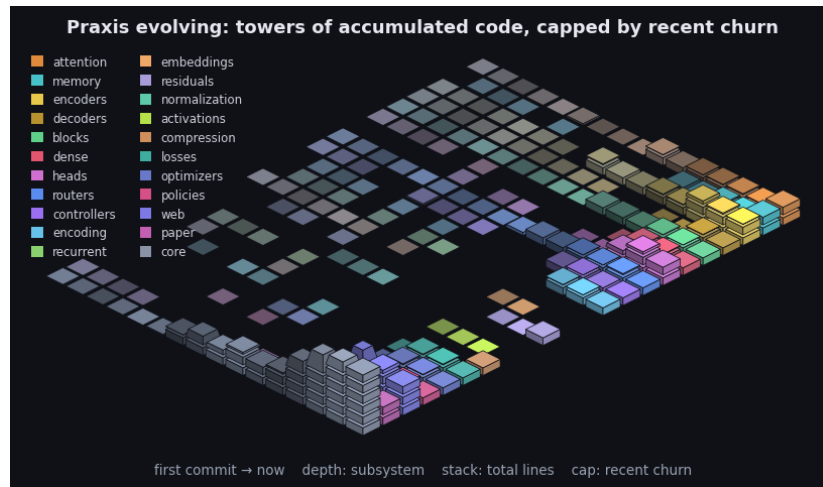
Figure 12: Praxis’s git history as an isometric terrain over the last 2490 commits. Each cell is one subsystem in one time window: a stack of base blocks for its accumulated size (total lines, recency-weighted) topped by a vivid cap for that window’s line churn - the standing codebase carrying the recent activity. Both are weighted by recency (the kernel the model applies to a sequence, turned on the repository): recent windows stack tall with bright caps while history thins toward the always-present prior - the low valley we roll into. Color fades from each subsystem’s hue toward a neutral prior into the past, banded in phased strata over a non-linear timescale. It is the bias/variance geometry read along the frequency axis (see the project notes): loud recent corrections over the quiet, ever-present base. By recency-weighted churn the current center of gravity is core, web, paper. The framework charts the hand that builds it.
