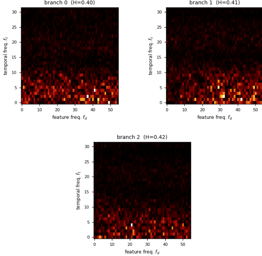
Figure 2: The static amplitude spectrum |a[f_t, f_d]| across the 3 arms of abstractinator-i’s prismatic head - the learned grid that, inverse-transformed through the frozen Weyl phases, becomes the bias field. This is the heatmap the text describes: energy that settles into a low-frequency band (small f_t, f_d ) is the corpus rhythm crystallizing, while a grid that stays uniform is a field still indistinguishable from noise. Hoyer concentrations H = 0.40, 0.41, 0.42 (left to right) quantifies it on the same [0, 1] scale the prose names (1 = a single cell, 0 = uniform), computed from this very tensor by concentration() - the same value the dashboard logs live. The pink 1/f^\alpha prior lives in the frozen basis, not in these amplitudes, so the grid shown is exactly what the head exposes.
