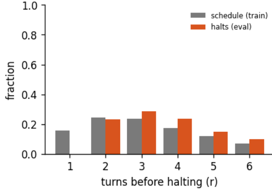
Figure 8: Halting distribution: the fraction of forward passes that stop after r turns, for the 6-turn recurrent loop of run abstractinator-i, early-halt rate 26%, mean boundary KL 0.285. schedule is the random loop-count the model trains under; halts is where the KL gate actually stops at inference. A mass pinned at the maximum (KL never collapsing) is the honest signature of a model that has not yet learned to converge early - the decision is real, not yet decisive.
