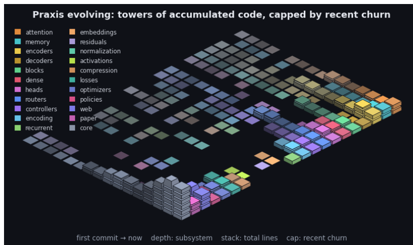
Figure 4: Praxis’s git history as an isometric terrain over the last 2246 commits. Each cell is one subsystem in one time window: a stack of base blocks for its accumulated size (total lines, recency-weighted) topped by a vivid cap for that window’s line churn - the standing codebase carrying the recent activity. Both are weighted by recency (the kernel the model applies to a sequence, turned on the repository): recent windows stack tall with bright caps while history thins toward the always-present prior - the low valley we roll into. Color fades from each subsystem’s hue toward a neutral prior into the past, banded in phased strata over a non-linear timescale. It is the bias/variance geometry read along the frequency axis (see the project notes): loud recent corrections over the quiet, ever-present base. By recency-weighted churn the current center of gravity is core, web, encoders. The framework charts the hand that builds it.
