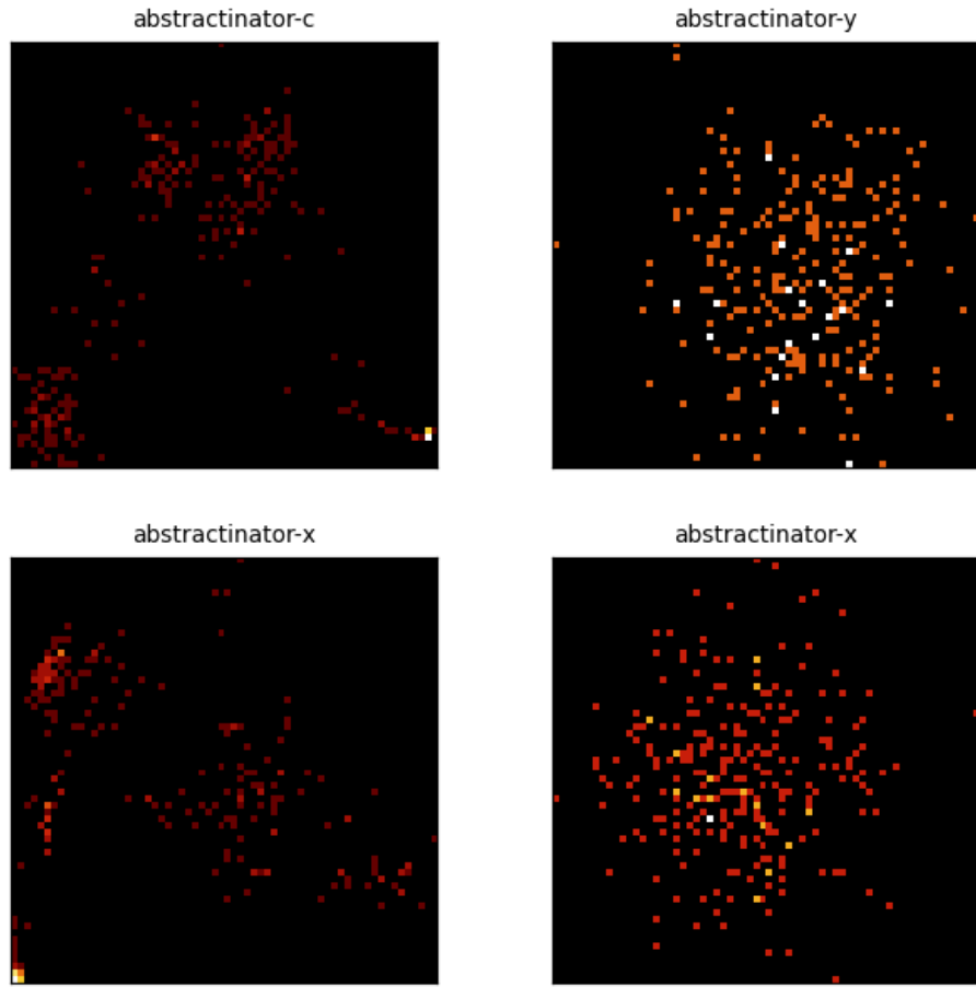
Figure 5: Center PCA density for the 4 most recent crystal-head runs (abstractinator-c, abstractinator-y, abstractinator-x, abstractinator-x). Each panel is the top-2 PCA projection of a head’s vocabulary centers, binned to a 64 \times 64 density grid (log color) - the same snapshot the dashboard renders live. Different runs settle into structurally different geometries, not noise.
