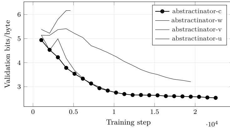
Figure 14: Bits per Byte across the 4 most recent experiments with comparable validation curves; the current experiment (abstractinator-c) is drawn in bold. Bold marks which run this build is reporting on , not which run scores best. The curves end wherever each run stopped, so they are at different points along their own training, and their endpoints are not a ranking. Generated from run logs - metrics that are not comparable across families (token loss vs. byte bits-per-byte vs. codec/CALM BrierLM) are excluded by construction, so the curves on this axis mean the same thing.
