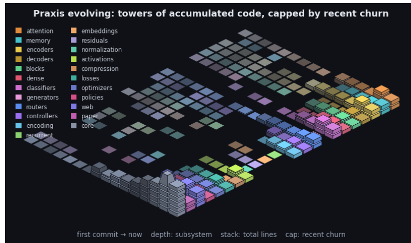
Figure 13: Praxis’s git history as an isometric terrain over the last 2644 commits. Each cell is one subsystem in one time window: a stack of base blocks for its accumulated size (total lines, recency-weighted) topped by a vivid cap for that window’s line churn - the standing codebase carrying the recent activity. Both are weighted by recency (the kernel the model applies to a sequence, turned on the repository): recent windows stack tall with bright caps while history thins toward the always-present prior - the low valley we roll into. Color fades from each subsystem’s hue toward a neutral prior into the past, banded in phased strata over a non-linear timescale. It is the bias/variance geometry read along the frequency axis (see the project notes): loud recent corrections over the quiet, ever-present base. By recency-weighted churn the current center of gravity is core, web, encoders. The framework charts the hand that builds it.
