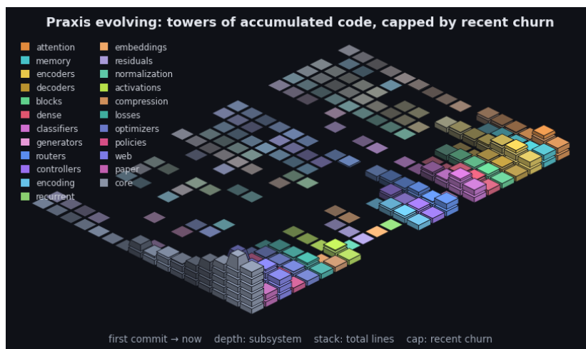
Figure 9: Praxis’s git history as an isometric terrain over the last 2690 commits. Each cell is one subsystem in one time window: a stack of base blocks for its accumulated size (total lines, recency-weighted) topped by a vivid cap for that window’s line churn - the standing codebase carrying the recent activity. Both are weighted by recency (the kernel the model applies to a sequence, turned on the repository): recent windows stack tall with bright caps while history thins toward the always-present prior - the low valley we roll into. Color fades from each subsystem’s hue toward a neutral prior into the past, banded in phased strata over a non-linear timescale. It is the bias/variance geometry read along the frequency axis (see the project notes): loud recent corrections over the quiet, ever-present base. By recency-weighted churn the current center of gravity is core, web, encoders. The framework charts the hand that builds it.
