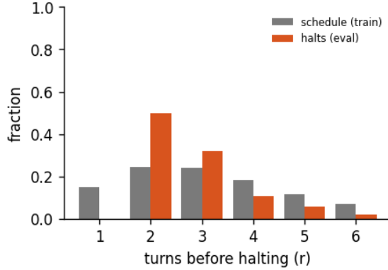
Figure 8: Halting distribution: the fraction of forward passes that stop after r turns, for the 6-turn recurrent loop of run abstractinator-g, early-halt rate 36%, mean boundary KL 0.347. schedule is the random loop-count the model trains under; halts is where the KL gate actually stops at inference. A mass pinned at the maximum (KL never collapsing) is the honest signature of a model that has not yet learned to converge early - the decision is real, not yet decisive.
