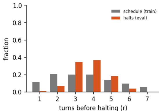
Figure 7: Halting distribution: the fraction of forward passes that stop after r turns, for the 7-turn recurrent loop of run abstractinator-c, early-halt rate 27%, mean boundary KL 0.247. schedule is the random loop-count the model trains under; halts is where the KL gate actually stops at inference. A mass pinned at the maximum (KL never collapsing) is the honest signature of a model that has not yet learned to converge early - the decision is real, not yet decisive.
