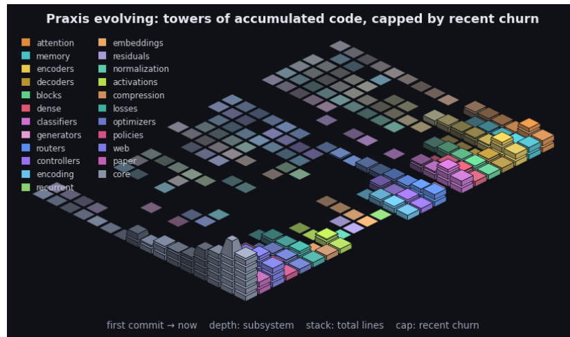
Figure 9: Praxis’s git history as an isometric terrain over the last 2625 commits. Each cell is one subsystem in one time window: a stack of base blocks for its accumulated size (total lines, recency-weighted) topped by a vivid cap for that window’s line churn - the standing codebase carrying the recent activity. Both are weighted by recency (the kernel the model applies to a sequence, turned on the repository): recent windows stack tall with bright caps while history thins toward the always-present prior - the low valley we roll into. Color fades from each subsystem’s hue toward a neutral prior into the past, banded in phased strata over a non-linear timescale. It is the bias/variance geometry read along the frequency axis (see the project notes): loud recent corrections over the quiet, ever-present base. By recency-weighted churn the current center of gravity is core, web, encoders. The framework charts the hand that builds it.
