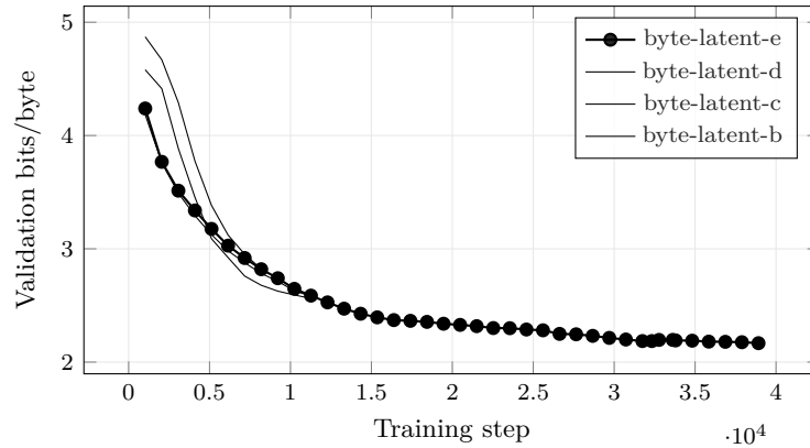
Figure 10: Bits per Byte across the 4 most recent experiments with comparable validation curves; the current experiment (byte-latent-e) is drawn in bold. Bold marks which run this build is reporting on , not which run scores best. The curves end wherever each run stopped, so they are at different points along their own training, and their endpoints are not a ranking. Generated from run logs - metrics that are not comparable across families (token loss vs. byte bits-per-byte vs. codec/CALM BrierLM) are excluded by construction, so the curves on this axis mean the same thing.
