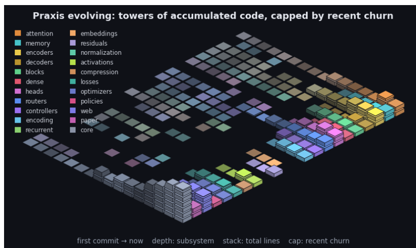
Figure 13: Praxis’s git history as an isometric terrain over the last 2583 commits. Each cell is one subsystem in one time window: a stack of base blocks for its accumulated size (total lines, recency-weighted) topped by a vivid cap for that window’s line churn - the standing codebase carrying the recent activity. Both are weighted by recency (the kernel the model applies to a sequence, turned on the repository): recent windows stack tall with bright caps while history thins toward the always-present prior - the low valley we roll into. Color fades from each subsystem’s hue toward a neutral prior into the past, banded in phased strata over a non-linear timescale. It is the bias/variance geometry read along the frequency axis (see the project notes): loud recent corrections over the quiet, ever-present base. By recency-weighted churn the current center of gravity is core, web, paper. The framework charts the hand that builds it.
