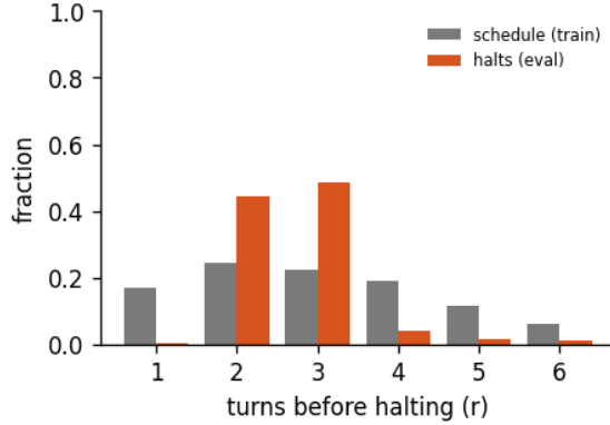
Figure 9: Halting distribution: the fraction of forward passes that stop after r turns, for the 6-turn recurrent loop of run abstractinator-q, early-halt rate 37%, mean boundary KL 0.225. schedule is the random loop-count the model trains under; halts is where the KL gate actually stops at inference. A mass pinned at the maximum (KL never collapsing) is the honest signature of a model that has not yet learned to converge early - the decision is real, not yet decisive.
