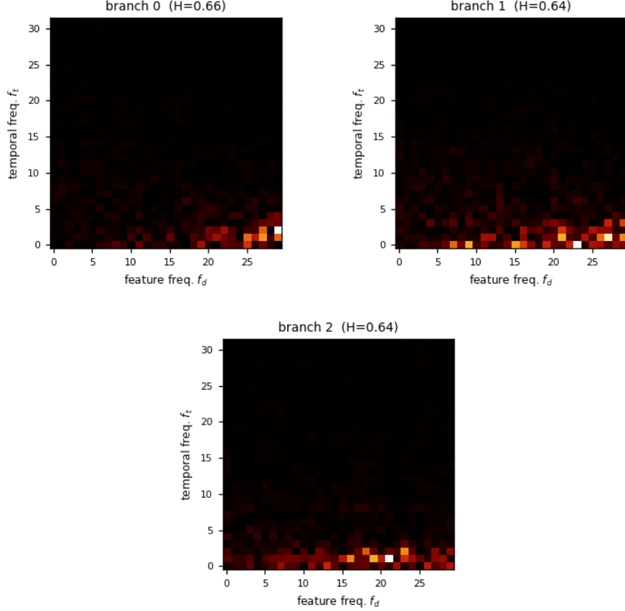
Figure 2: The static amplitude spectrum |a[f_t, f_d]| across the 3 arms of abstractinator-d’s prismatic head - the learned grid that, inverse-transformed through the frozen Weyl phases, becomes the bias field. This is the heatmap the text describes: energy that settles into a low-frequency band (small f_t, f_d ) is the corpus rhythm crystallizing, while a grid that stays uniform is a field still indistinguishable from noise. Hoyer concentrations H = 0.66, 0.64, 0.64 (left to right) quantifies it on the same [0, 1] scale the prose names (1 = a single cell, 0 = uniform), computed from this very tensor by concentration() - the same value the dashboard logs live. The pink 1/f^\alpha prior lives in the frozen basis, not in these amplitudes, so the grid shown is exactly what the head exposes.
