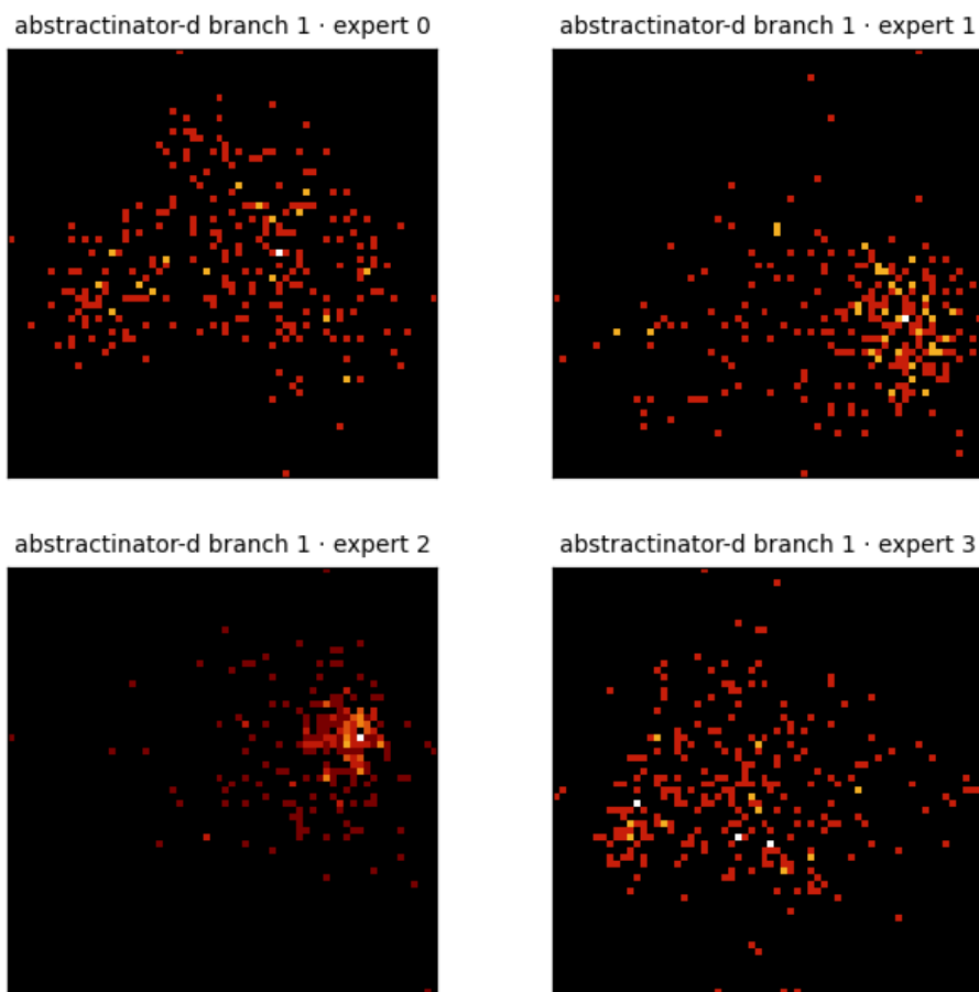
Figure 11: Center PCA density for the 4 crystal heads of abstractinator-d - a single multi-head model (prismatic4’s VEAR crystal bank), so these are that run’s own heads (branch 1 · expert 0, branch 1 · expert 1, branch 1 · expert 2, branch 1 · expert 3), not a cross-run mix. Each panel is the top-2 PCA projection of a head’s vocabulary centers, binned to a 64 \times 64 density grid (log color) - the same snapshot the dashboard renders live. The bank’s experts settle into structurally distinct geometries - the between-expert variance the router selects over.
