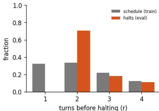
Figure 8: Halting distribution: the fraction of forward passes that stop after r turns, for the 4-turn recurrent loop of run abstractinator-e, early-halt rate 39%, mean boundary KL 0.381. schedule is the random loop-count the model trains under; halts is where the KL gate actually stops at inference. A mass pinned at the maximum (KL never collapsing) is the honest signature of a model that has not yet learned to converge early - the decision is real, not yet decisive.
