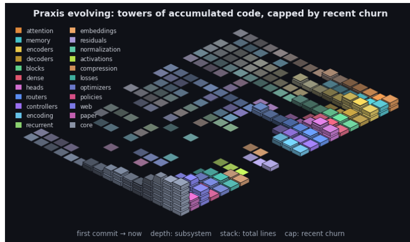
Figure 12: Praxis’s git history as an isometric terrain over the last 2437 commits. Each cell is one subsystem in one time window: a stack of base blocks for its accumulated size (total lines, recency-weighted) topped by a vivid cap for that window’s line churn - the standing codebase carrying the recent activity. Both are weighted by recency (the kernel the model applies to a sequence, turned on the repository): recent windows stack tall with bright caps while history thins toward the always-present prior - the low valley we roll into. Color fades from each subsystem’s hue toward a neutral prior into the past, banded in phased strata over a non-linear timescale. It is the bias/variance geometry read along the frequency axis (see the project notes): loud recent corrections over the quiet, ever-present base. By recency-weighted churn the current center of gravity is core, web, paper. The framework charts the hand that builds it.
