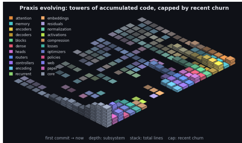
Figure 10: Praxis’s git history as an isometric terrain over the last 2403 commits. Each cell is one subsystem in one time window: a stack of base blocks for its accumulated size (total lines, recency-weighted) topped by a vivid cap for that window’s line churn - the standing codebase carrying the recent activity. Both are weighted by recency (the kernel the model applies to a sequence, turned on the repository): recent windows stack tall with bright caps while history thins toward the always-present prior - the low valley we roll into. Color fades from each subsystem’s hue toward a neutral prior into the past, banded in phased strata over a non-linear timescale. It is the bias/variance geometry read along the frequency axis (see the project notes): loud recent corrections over the quiet, ever-present base. By recency-weighted churn the current center of gravity is core, web, paper. The framework charts the hand that builds it.
