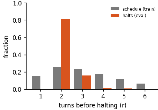
Figure 9: Halting distribution: the fraction of forward passes that stop after r turns, for the 6-turn recurrent loop of run abstractinator-j, early-halt rate 45%, mean boundary KL 1.01. schedule is the random loop-count the model trains under; halts is where the KL gate actually stops at inference. A mass pinned at the maximum (KL never collapsing) is the honest signature of a model that has not yet learned to converge early - the decision is real, not yet decisive.
