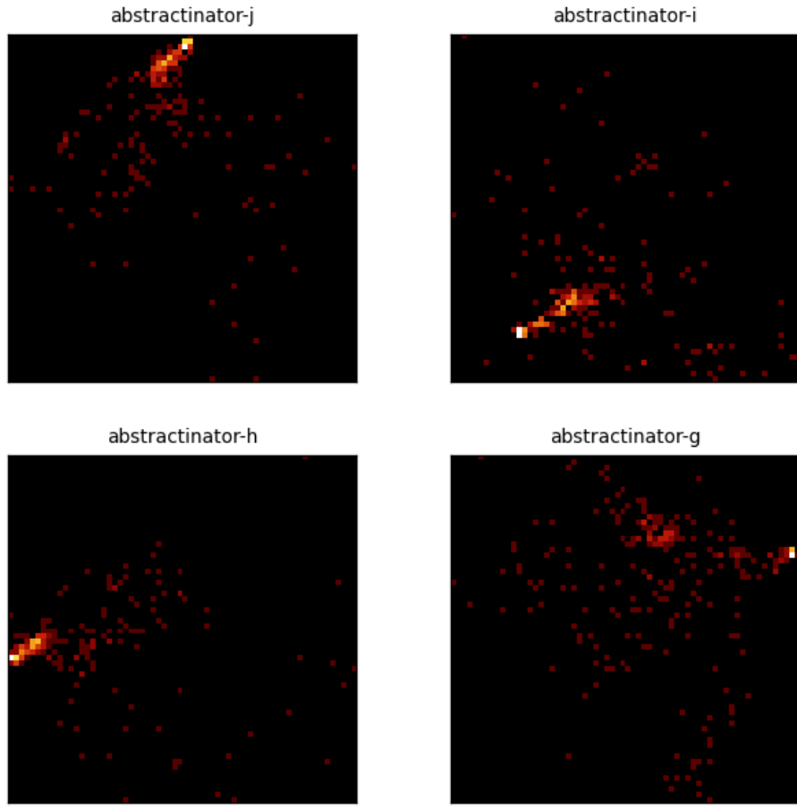
Figure 12: Center PCA density for the 4 most recent crystal-head runs (abstractinator-j, abstractinator-i, abstractinator-h, abstractinator-g). Each panel is the top-2 PCA projection of a head’s vocabulary centers, binned to a 64 \times 64 density grid (log color) - the same snapshot the dashboard renders live. Different runs settle into structurally different geometries, not noise.
