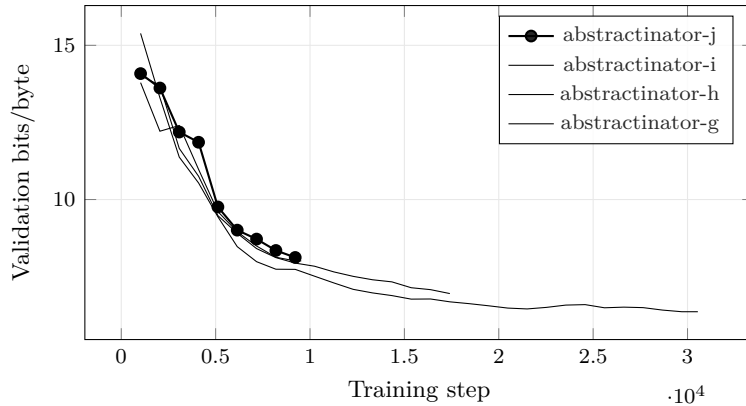
Figure 14: Bits per Byte across the 4 most recent experiments with comparable validation curves; the current experiment (abstractinator-j) is drawn in bold. Bold marks which run this build is reporting on , not which run scores best. The curves end wherever each run stopped, so they are at different points along their own training, and their endpoints are not a ranking. Generated from run logs - metrics that are not comparable across families (token loss vs. byte bits-per-byte vs. codec/CALM BrierLM) are excluded by construction, so the curves on this axis mean the same thing.
