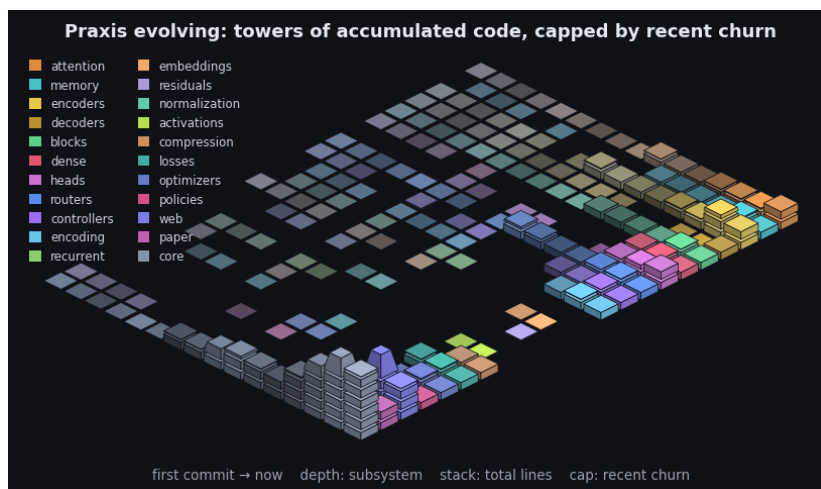
Figure 9: Praxis’s git history as an isometric terrain over the last 2364 commits. Each cell is one subsystem in one time window: a stack of base blocks for its accumulated size (total lines, recency-weighted) topped by a vivid cap for that window’s line churn - the standing codebase carrying the recent activity. Both are weighted by recency (the kernel the model applies to a sequence, turned on the repository): recent windows stack tall with bright caps while history thins toward the always-present prior - the low valley we roll into. Color fades from each subsystem’s hue toward a neutral prior into the past, banded in phased strata over a non-linear timescale. It is the bias/variance geometry read along the frequency axis (see the project notes): loud recent corrections over the quiet, ever-present base. By recency-weighted churn the current center of gravity is core, web, paper. The framework charts the hand that builds it.
