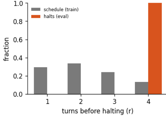
Figure 5: Halting distribution: the fraction of forward passes that stop after r turns, for the 4-turn recurrent loop of run calm-d, early-halt rate 0%, mean boundary KL 163. schedule is the random loop-count the model trains under; halts is where the KL gate actually stops at inference. A mass pinned at the maximum (KL never collapsing) is the honest signature of a model that has not yet learned to converge early - the decision is real, not yet decisive.
