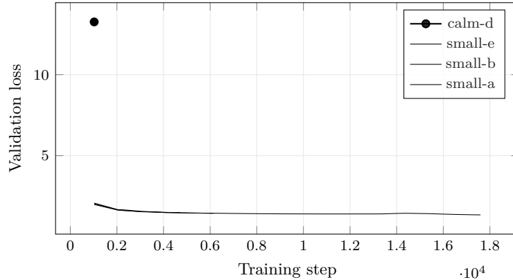
Figure 8: Validation Loss across the 4 most recent experiments with comparable validation curves; the leading run (calm-d) is drawn in bold. Generated from run logs - metrics that are not comparable across families (token loss vs. byte bits-per-byte vs. codec/CALM BrierLM) are excluded by construction, so the curves on this axis mean the same thing.
