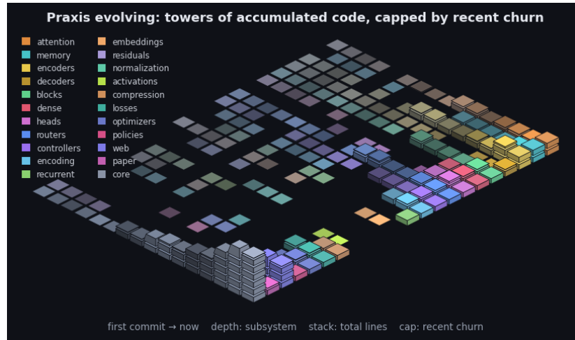
Figure 7: Praxis’s git history as an isometric terrain over the last 2215 commits. Each cell is one subsystem in one time window: a stack of base blocks for its accumulated size (total lines, recency-weighted) topped by a vivid cap for that window’s line churn - the standing codebase carrying the recent activity. Both are weighted by recency (the kernel the model applies to a sequence, turned on the repository): recent windows stack tall with bright caps while history thins toward the always-present prior - the low valley we roll into. Color fades from each subsystem’s hue toward a neutral prior into the past, banded in phased strata over a non-linear timescale. It is the bias/variance geometry read along the frequency axis (see the project notes): loud recent corrections over the quiet, ever-present base. By recency-weighted churn the current center of gravity is core, web, encoders. The framework charts the hand that builds it.
