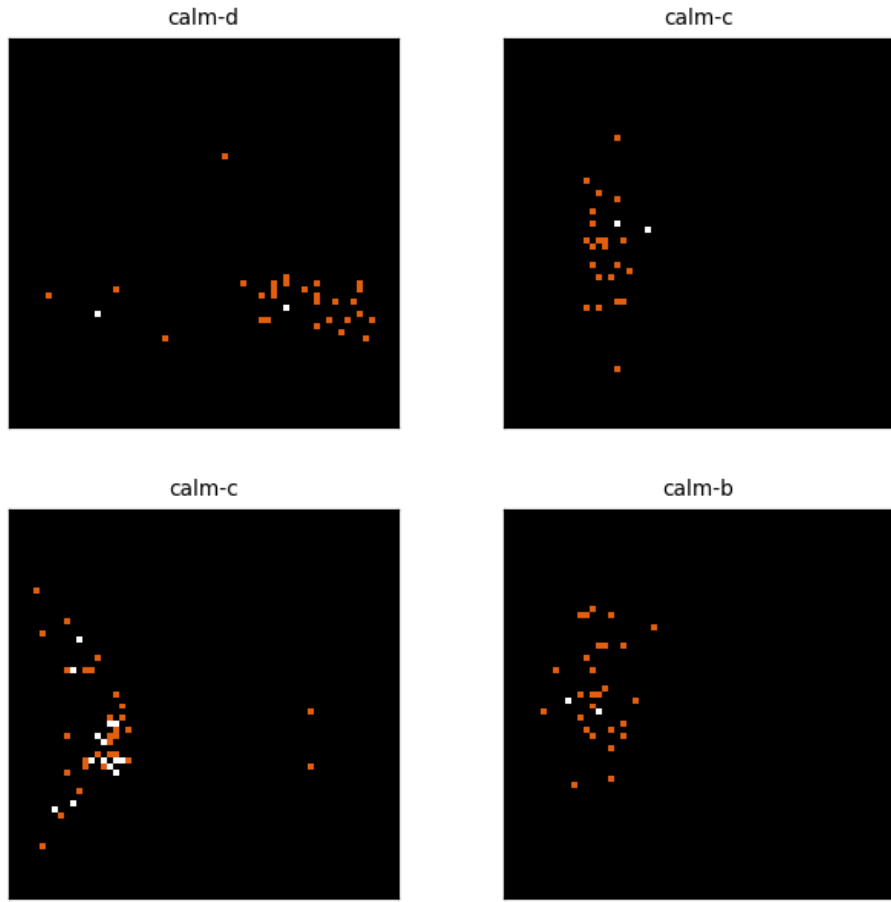
Figure 2: Center PCA density for the 4 most recent crystal-head runs (calm-d, calm-c, calm-c, calm-b). Each panel is the top-2 PCA projection of a head's vocabulary centers, binned to a 64 \times 64 density grid (log color) - the same snapshot the dashboard renders live. Different runs settle into structurally different geometries, not noise.
