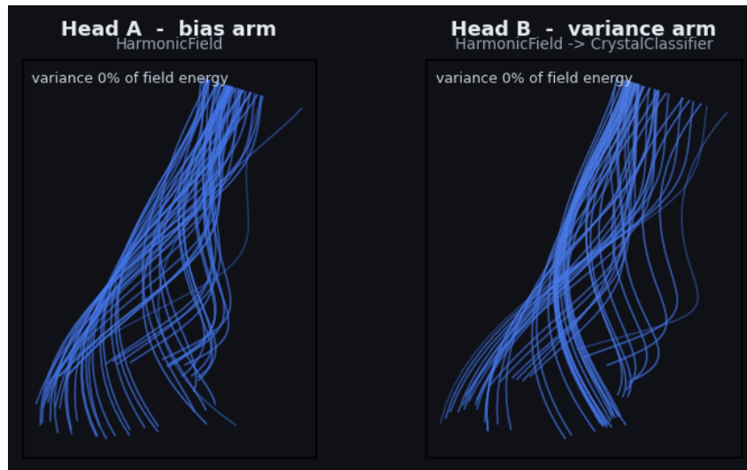
Figure 4: The prismatic head's two arms, rendered exactly as the dashboard's bias/variance strand card. Each hair is one feature, morphing from a ring (its static-field phase) out to its (bias, variance) position with a helical twist; color runs blue (pure bias) to red (pure variance). Head A (left) is the bias arm: it reads a static field, so every hair stays blue - a constant structural vote. Head B (right) is the variance arm, whose input-conditional envelope lets hairs swing toward red - the data-dependent vote. Each panel's subtitle lists that arm's head stack. The two together are the orthogonal bias/variance decomposition made architectural - convex and radial from the center, chaotic in the arms.
