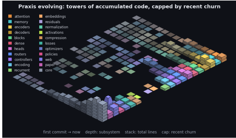
Figure 4: Praxis’s git history as an isometric terrain over the last 2337 commits. Each cell is one subsystem in one time window: a stack of base blocks for its accumulated size (total lines, recency-weighted) topped by a vivid cap for that window’s line churn - the standing codebase carrying the recent activity. Both are weighted by recency (the kernel the model applies to a sequence, turned on the repository): recent windows stack tall with bright caps while history thins toward the always-present prior - the low valley we roll into. Color fades from each subsystem’s hue toward a neutral prior into the past, banded in phased strata over a non-linear timescale. It is the bias/variance geometry read along the frequency axis (see the project notes): loud recent corrections over the quiet, ever-present base. By recency-weighted churn the current center of gravity is core, web, paper. The framework charts the hand that builds it.
