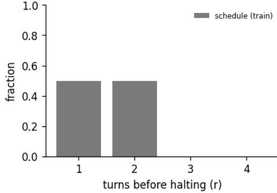
Figure 2: Halting distribution: the fraction of forward passes that stop after r turns, for the 4-turn recurrent loop of run calm-d. schedule is the random loop-count the model trains under; halts is where the KL gate actually stops at inference. A mass pinned at the maximum (KL never collapsing) is the honest signature of a model that has not yet learned to converge early - the decision is real, not yet decisive.
