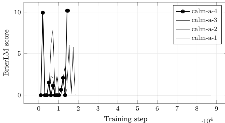
Figure 5: BrierLM across the 4 most recent experiments with comparable validation curves; the leading run (calm-a-4) is drawn in bold. Generated from run logs - metrics that are not comparable across families (token loss vs. byte bits-per-byte vs. codec/CALM BrierLM) are excluded by construction, so the curves on this axis mean the same thing.
