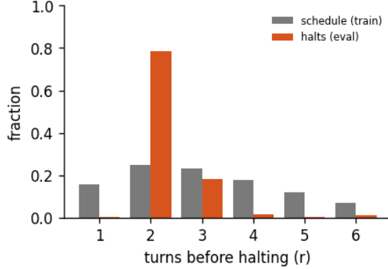
Figure 9: Halting distribution: the fraction of forward passes that stop after r turns, for the 6-turn recurrent loop of run abstractinator-o, early-halt rate 44%, mean boundary KL 0.999. schedule is the random loop-count the model trains under; halts is where the KL gate actually stops at inference. A mass pinned at the maximum (KL never collapsing) is the honest signature of a model that has not yet learned to converge early - the decision is real, not yet decisive.
