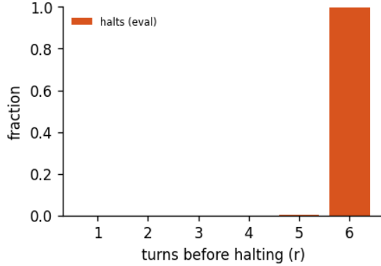
Figure 5: Halting distribution: the fraction of forward passes that stop after r turns, for the 6-turn recurrent loop of run calm-d, early-halt rate 0%, mean boundary KL 145. schedule is the random loop-count the model trains under; halts is where the KL gate actually stops at inference. A mass pinned at the maximum (KL never collapsing) is the honest signature of a model that has not yet learned to converge early - the decision is real, not yet decisive.
