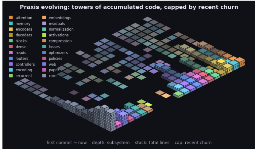
Figure 7: Praxis’s git history as an isometric terrain over the last 2231 commits. Each cell is one subsystem in one time window: a stack of base blocks for its accumulated size (total lines, recency-weighted) topped by a vivid cap for that window’s line churn - the standing codebase carrying the recent activity. Both are weighted by recency (the kernel the model applies to a sequence, turned on the repository): recent windows stack tall with bright caps while history thins toward the always-present prior - the low valley we roll into. Color fades from each subsystem’s hue toward a neutral prior into the past, banded in phased strata over a non-linear timescale. It is the bias/variance geometry read along the frequency axis (see the project notes): loud recent corrections over the quiet, ever-present base. By recency-weighted churn the current center of gravity is core, web, encoders. The framework charts the hand that builds it.
