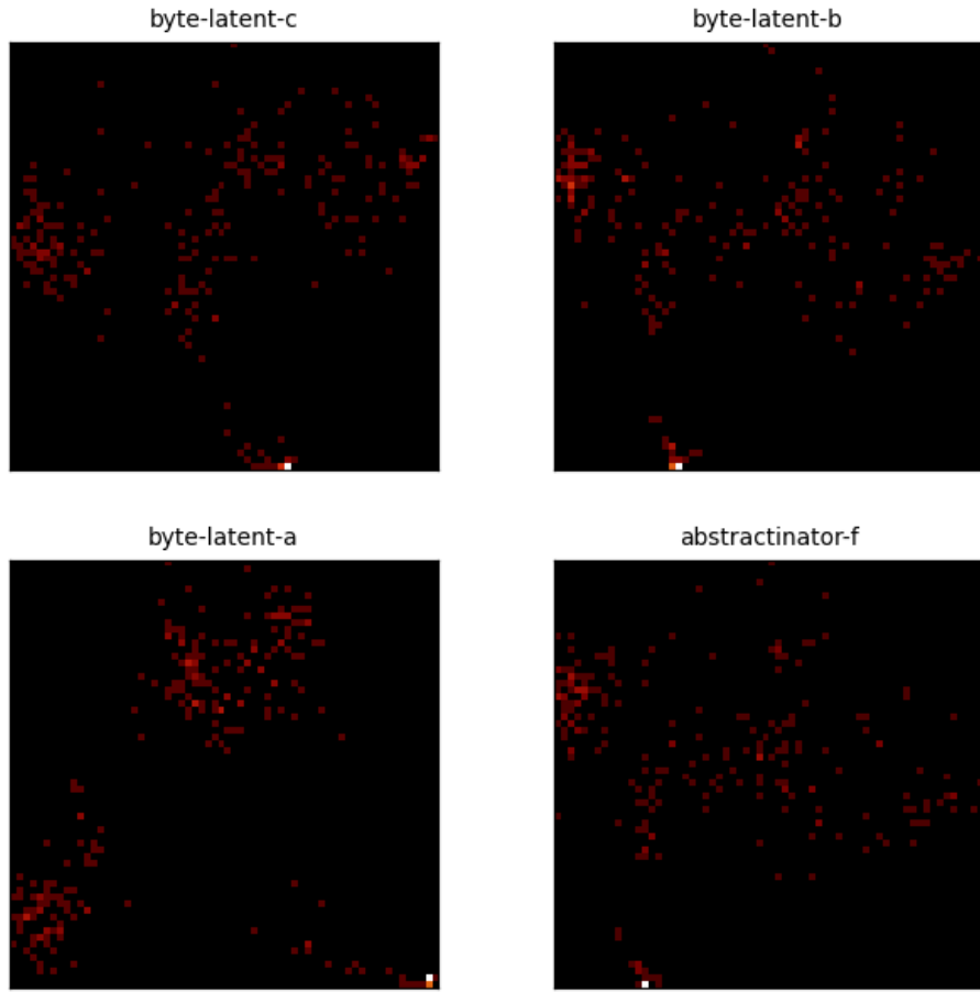
Figure 8: Center PCA density for the 4 most recent crystal-head runs ( byte-latent-c , byte-latent-b , byte-latent-a , abstractinator-f ). Each panel is the top-2 PCA projection of a head’s vocabulary centers, binned to a 64 \times 64 density grid (log color) - the same snapshot the dashboard renders live. Different runs settle into structurally different geometries, not noise.
