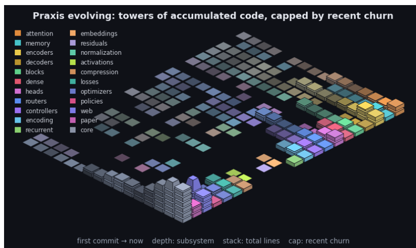
Figure 4: Praxis’s git history as an isometric terrain over the last 2315 commits. Each cell is one subsystem in one time window: a stack of base blocks for its accumulated size (total lines, recency-weighted) topped by a vivid cap for that window’s line churn - the standing codebase carrying the recent activity. Both are weighted by recency (the kernel the model applies to a sequence, turned on the repository): recent windows stack tall with bright caps while history thins toward the always-present prior - the low valley we roll into. Color fades from each subsystem’s hue toward a neutral prior into the past, banded in phased strata over a non-linear timescale. It is the bias/variance geometry read along the frequency axis (see the project notes): loud recent corrections over the quiet, ever-present base. By recency-weighted churn the current center of gravity is core, web, paper. The framework charts the hand that builds it.
