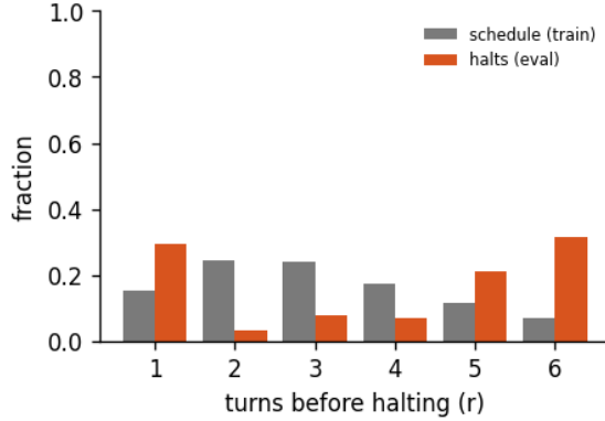
Figure 9: Halting distribution: the fraction of forward passes that stop after r turns, for the 6-turn recurrent loop of run byte-latent-a, early-halt rate 20%, mean boundary KL 0.0177. schedule is the random loop-count the model trains under; halts is where the KL gate actually stops at inference. A mass pinned at the maximum (KL never collapsing) is the honest signature of a model that has not yet learned to converge early - the decision is real, not yet decisive.
