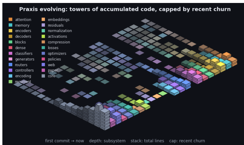
Figure 13: Praxis’s git history as an isometric terrain over the last 2646 commits. Each cell is one subsystem in one time window: a stack of base blocks for its accumulated size (total lines, recency-weighted) topped by a vivid cap for that window’s line churn - the standing codebase carrying the recent activity. Both are weighted by recency (the kernel the model applies to a sequence, turned on the repository): recent windows stack tall with bright caps while history thins toward the always-present prior - the low valley we roll into. Color fades from each subsystem’s hue toward a neutral prior into the past, banded in phased strata over a non-linear timescale. It is the bias/variance geometry read along the frequency axis (see the project notes): loud recent corrections over the quiet, ever-present base. By recency-weighted churn the current center of gravity is core, web, encoders. The framework charts the hand that builds it.
