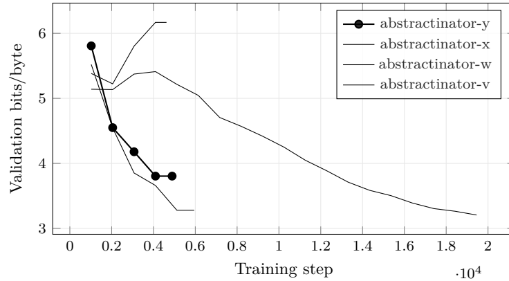
Figure 10: Bits per Byte across the 4 most recent experiments with comparable validation curves; the current experiment (abstractinator-y) is drawn in bold. Bold marks which run this build is reporting on , not which run scores best. The curves end wherever each run stopped, so they are at different points along their own training, and their endpoints are not a ranking. Generated from run logs - metrics that are not comparable across families (token loss vs. byte bits-per-byte vs. codec/CALM BrierLM) are excluded by construction, so the curves on this axis mean the same thing.
