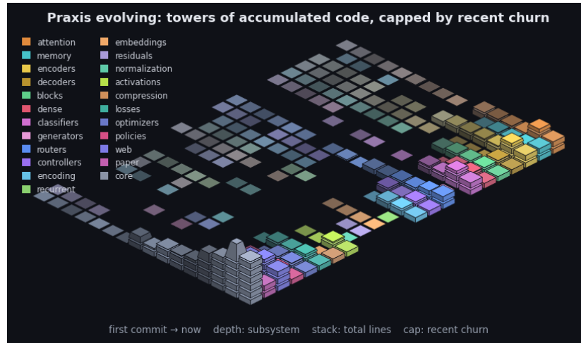
Figure 9: Praxis’s git history as an isometric terrain over the last 2624 commits. Each cell is one subsystem in one time window: a stack of base blocks for its accumulated size (total lines, recency-weighted) topped by a vivid cap for that window’s line churn - the standing codebase carrying the recent activity. Both are weighted by recency (the kernel the model applies to a sequence, turned on the repository): recent windows stack tall with bright caps while history thins toward the always-present prior - the low valley we roll into. Color fades from each subsystem’s hue toward a neutral prior into the past, banded in phased strata over a non-linear timescale. It is the bias/variance geometry read along the frequency axis (see the project notes): loud recent corrections over the quiet, ever-present base. By recency-weighted churn the current center of gravity is core, web, encoders. The framework charts the hand that builds it.
