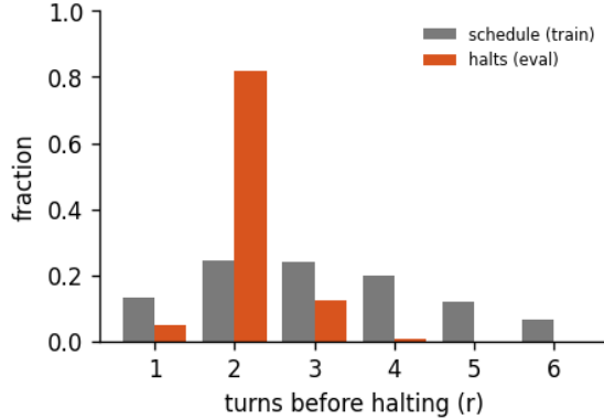
Figure 9: Halting distribution: the fraction of forward passes that stop after r turns, for the 6-turn recurrent loop of run byte-latent-a, early-halt rate 48%, mean boundary KL 0.0429. schedule is the random loop-count the model trains under; halts is where the KL gate actually stops at inference. A mass pinned at the maximum (KL never collapsing) is the honest signature of a model that has not yet learned to converge early - the decision is real, not yet decisive.
