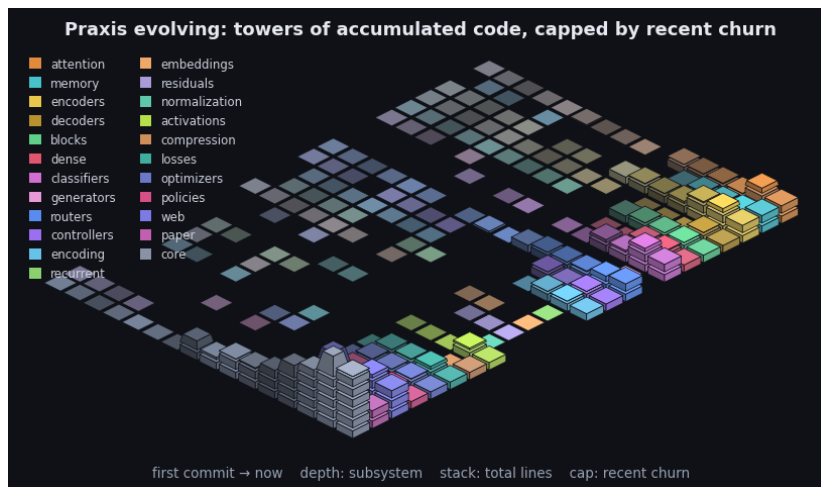
Figure 9: Praxis’s git history as an isometric terrain over the last 2666 commits. Each cell is one subsystem in one time window: a stack of base blocks for its accumulated size (total lines, recency-weighted) topped by a vivid cap for that window’s line churn - the standing codebase carrying the recent activity. Both are weighted by recency (the kernel the model applies to a sequence, turned on the repository): recent windows stack tall with bright caps while history thins toward the always-present prior - the low valley we roll into. Color fades from each subsystem’s hue toward a neutral prior into the past, banded in phased strata over a non-linear timescale. It is the bias/variance geometry read along the frequency axis (see the project notes): loud recent corrections over the quiet, ever-present base. By recency-weighted churn the current center of gravity is core, web, encoders. The framework charts the hand that builds it.
