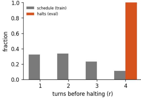
Figure 2: Halting distribution: the fraction of forward passes that stop after r turns, for the 4-turn recurrent loop of run calm-e, early-halt rate 0%, mean boundary KL 10.2. schedule is the random loop-count the model trains under; halts is where the KL gate actually stops at inference. A mass pinned at the maximum (KL never collapsing) is the honest signature of a model that has not yet learned to converge early - the decision is real, not yet decisive.
