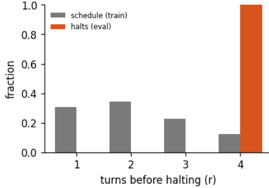
Figure 4: Halting distribution: the fraction of forward passes that stop after r turns, for the 4-turn recurrent loop of run calm-e, early-halt rate 0%, mean boundary KL 95.5. schedule is the random loop-count the model trains under; halts is where the KL gate actually stops at inference. A mass pinned at the maximum (KL never collapsing) is the honest signature of a model that has not yet learned to converge early - the decision is real, not yet decisive.
