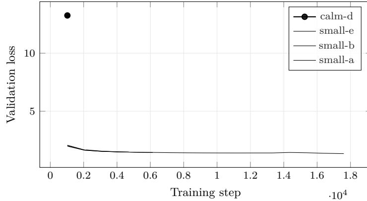
Figure 7: Validation Loss across the 4 most recent experiments with comparable validation curves; the leading run (calm-d) is drawn in bold. Generated from run logs - metrics that are not comparable across families (token loss vs. byte bits-per-byte vs. codec/CALM BrierLM) are excluded by construction, so the curves on this axis mean the same thing.
