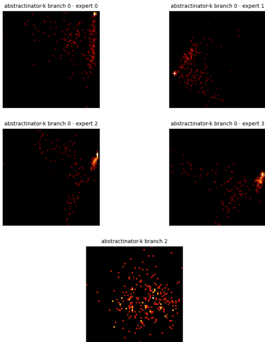
Figure 11: Center PCA density for the 5 crystal heads of abstractinator-k - a single multi-head model (prismatic4’s VEAR crystal bank), so these are that run’s own heads (branch 0 · expert 0, branch 0 · expert 1, branch 0 · expert 2, branch 0 · expert 3, branch 2), not a cross-run mix. Each panel is the top-2 PCA projection of a head’s vocabulary centers, binned to a 64 \times 64 density grid (log color) - the same snapshot the dashboard renders live. The bank’s experts settle into structurally distinct geometries - the between-expert variance the router selects over.
