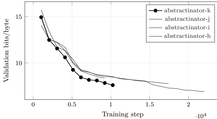
Figure 13: Bits per Byte across the 4 most recent experiments with comparable validation curves; the current experiment (abstractinator-k) is drawn in bold. Bold marks which run this build is reporting on , not which run scores best. The curves end wherever each run stopped, so they are at different points along their own training, and their endpoints are not a ranking. Generated from run logs - metrics that are not comparable across families (token loss vs. byte bits-per-byte vs. codec/CALM BrierLM) are excluded by construction, so the curves on this axis mean the same thing.
