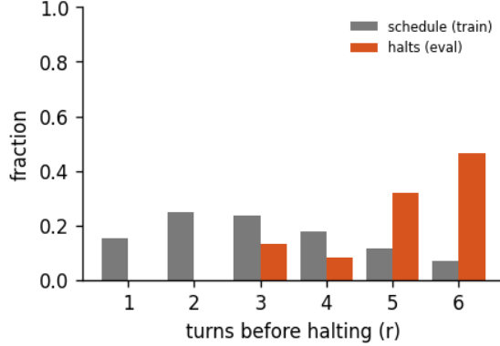
Figure 8: Halting distribution: the fraction of forward passes that stop after r turns, for the 6-turn recurrent loop of run abstractinator-k, early-halt rate 11%, mean boundary KL 0.425. schedule is the random loop-count the model trains under; halts is where the KL gate actually stops at inference. A mass pinned at the maximum (KL never collapsing) is the honest signature of a model that has not yet learned to converge early - the decision is real, not yet decisive.
