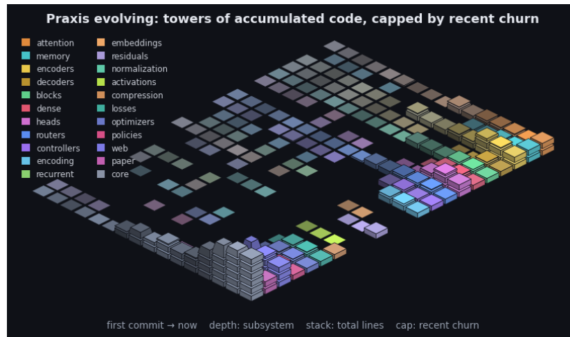
Figure 12: Praxis’s git history as an isometric terrain over the last 2502 commits. Each cell is one subsystem in one time window: a stack of base blocks for its accumulated size (total lines, recency-weighted) topped by a vivid cap for that window’s line churn - the standing codebase carrying the recent activity. Both are weighted by recency (the kernel the model applies to a sequence, turned on the repository): recent windows stack tall with bright caps while history thins toward the always-present prior - the low valley we roll into. Color fades from each subsystem’s hue toward a neutral prior into the past, banded in phased strata over a non-linear timescale. It is the bias/variance geometry read along the frequency axis (see the project notes): loud recent corrections over the quiet, ever-present base. By recency-weighted churn the current center of gravity is core, web, paper. The framework charts the hand that builds it.
