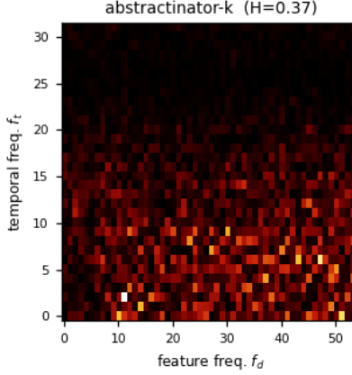
Figure 2: The static amplitude spectrum |a[f_t, f_d]| for abstractinator-k - the learned grid that, inverse-transformed through the frozen Weyl phases, becomes the bias field. This is the heatmap the text describes: energy that settles into a low-frequency band (small f_t, f_d ) is the corpus rhythm crystallizing, while a grid that stays uniform is a field still indistinguishable from noise. Hoyer concentration H = 0.37 quantifies it on the same [0, 1] scale the prose names (1 = a single cell, 0 = uniform), computed from this very tensor by concentration() - the same value the dashboard logs live. The pink 1/f^\alpha prior lives in the frozen basis, not in these amplitudes, so the grid shown is exactly what the head exposes.
