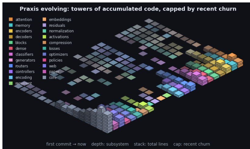
Figure 9: Praxis’s git history as an isometric terrain over the last 2680 commits. Each cell is one subsystem in one time window: a stack of base blocks for its accumulated size (total lines, recency-weighted) topped by a vivid cap for that window’s line churn - the standing codebase carrying the recent activity. Both are weighted by recency (the kernel the model applies to a sequence, turned on the repository): recent windows stack tall with bright caps while history thins toward the always-present prior - the low valley we roll into. Color fades from each subsystem’s hue toward a neutral prior into the past, banded in phased strata over a non-linear timescale. It is the bias/variance geometry read along the frequency axis (see the project notes): loud recent corrections over the quiet, ever-present base. By recency-weighted churn the current center of gravity is core, web, encoders. The framework charts the hand that builds it.
