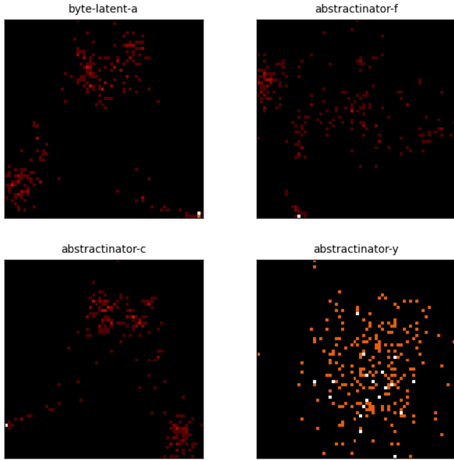
Figure 11: Center PCA density for the 4 most recent crystal-head runs (byte-latent-a, abstractinator-f, abstractinator-c, abstractinator-y). Each panel is the top-2 PCA projection of a head’s vocabulary centers, binned to a 64 \times 64 density grid (log color) - the same snapshot the dashboard renders live. Different runs settle into structurally different geometries, not noise.
