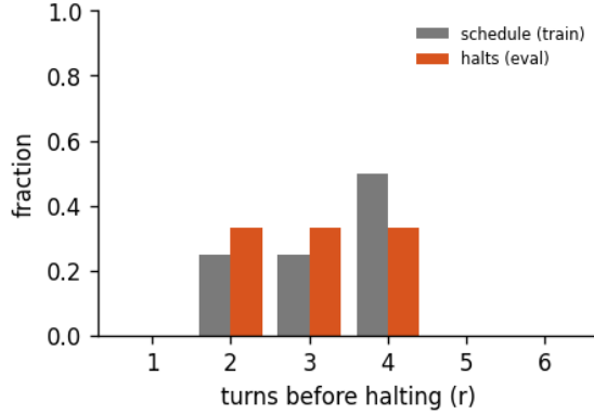
Figure 8: Halting distribution: the fraction of forward passes that stop after r turns, for the 6-turn recurrent loop of run byte-latent-b, early-halt rate 33%, mean boundary KL 0.0798. schedule is the random loop-count the model trains under; halts is where the KL gate actually stops at inference. A mass pinned at the maximum (KL never collapsing) is the honest signature of a model that has not yet learned to converge early - the decision is real, not yet decisive.
