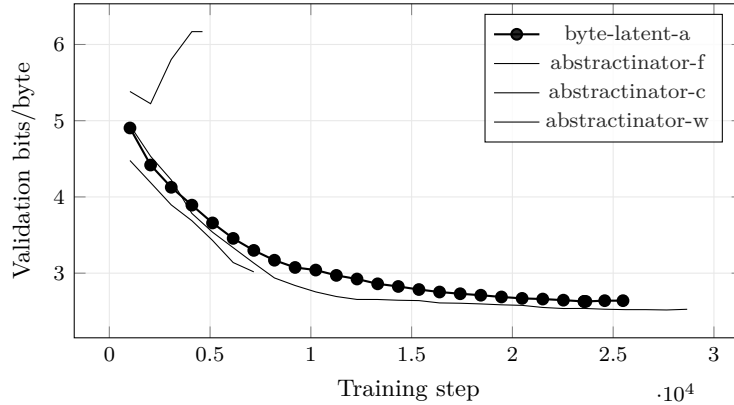
Figure 13: Bits per Byte across the 4 most recent experiments with comparable validation curves; the current experiment (byte-latent-a) is drawn in bold. Bold marks which run this build is reporting on , not which run scores best. The curves end wherever each run stopped, so they are at different points along their own training, and their endpoints are not a ranking. Generated from run logs - metrics that are not comparable across families (token loss vs. byte bits-per-byte vs. codec/CALM BrierLM) are excluded by construction, so the curves on this axis mean the same thing.
