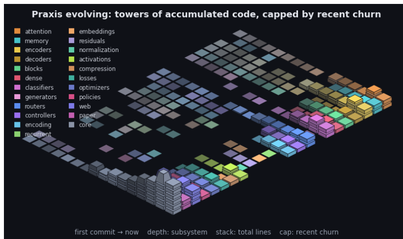
Figure 12: Praxis’s git history as an isometric terrain over the last 2662 commits. Each cell is one subsystem in one time window: a stack of base blocks for its accumulated size (total lines, recency-weighted) topped by a vivid cap for that window’s line churn - the standing codebase carrying the recent activity. Both are weighted by recency (the kernel the model applies to a sequence, turned on the repository): recent windows stack tall with bright caps while history thins toward the always-present prior - the low valley we roll into. Color fades from each subsystem’s hue toward a neutral prior into the past, banded in phased strata over a non-linear timescale. It is the bias/variance geometry read along the frequency axis (see the project notes): loud recent corrections over the quiet, ever-present base. By recency-weighted churn the current center of gravity is core, web, encoders. The framework charts the hand that builds it.
