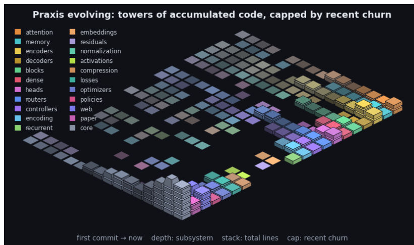
Figure 4: Praxis’s git history as an isometric terrain over the last 2288 commits. Each cell is one subsystem in one time window: a stack of base blocks for its accumulated size (total lines, recency-weighted) topped by a vivid cap for that window’s line churn - the standing codebase carrying the recent activity. Both are weighted by recency (the kernel the model applies to a sequence, turned on the repository): recent windows stack tall with bright caps while history thins toward the always-present prior - the low valley we roll into. Color fades from each subsystem’s hue toward a neutral prior into the past, banded in phased strata over a non-linear timescale. It is the bias/variance geometry read along the frequency axis (see the project notes): loud recent corrections over the quiet, ever-present base. By recency-weighted churn the current center of gravity is core, web, encoders. The framework charts the hand that builds it.
