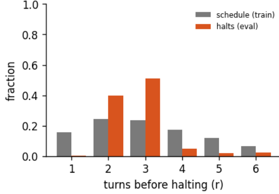
Figure 8: Halting distribution: the fraction of forward passes that stop after r turns, for the 6-turn recurrent loop of run abstractinator-q, early-halt rate 36%, mean boundary KL 0.159. schedule is the random loop-count the model trains under; halts is where the KL gate actually stops at inference. A mass pinned at the maximum (KL never collapsing) is the honest signature of a model that has not yet learned to converge early - the decision is real, not yet decisive.
