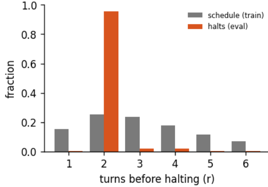
Figure 9: Halting distribution: the fraction of forward passes that stop after r turns, for the 6-turn recurrent loop of run abstractinator-u, early-halt rate 48%, mean boundary KL 0.892. schedule is the random loop-count the model trains under; halts is where the KL gate actually stops at inference. A mass pinned at the maximum (KL never collapsing) is the honest signature of a model that has not yet learned to converge early - the decision is real, not yet decisive.
