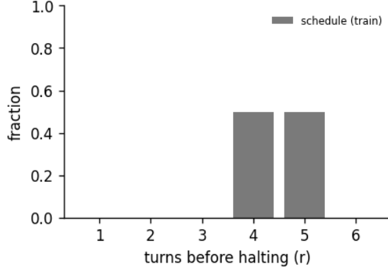
Figure 9: Halting distribution: the fraction of forward passes that stop after r turns, for the 6-turn recurrent loop of run abstractinator-v. schedule is the random loop-count the model trains under; halts is where the KL gate actually stops at inference. A mass pinned at the maximum (KL never collapsing) is the honest signature of a model that has not yet learned to converge early - the decision is real, not yet decisive.
