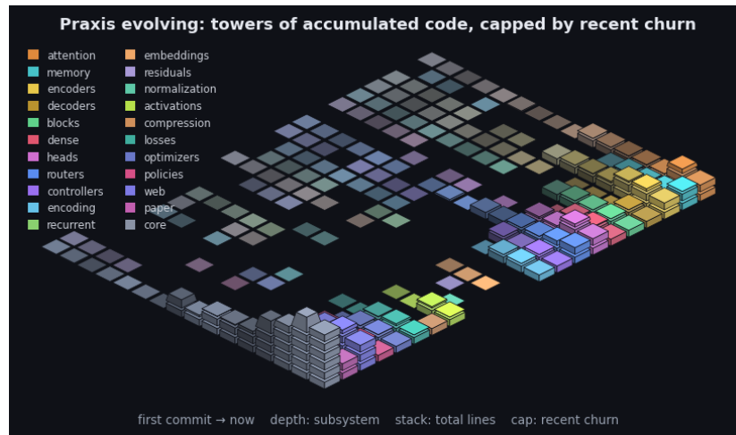
Figure 13: Praxis’s git history as an isometric terrain over the last 2606 commits. Each cell is one subsystem in one time window: a stack of base blocks for its accumulated size (total lines, recency-weighted) topped by a vivid cap for that window’s line churn - the standing codebase carrying the recent activity. Both are weighted by recency (the kernel the model applies to a sequence, turned on the repository): recent windows stack tall with bright caps while history thins toward the always-present prior - the low valley we roll into. Color fades from each subsystem’s hue toward a neutral prior into the past, banded in phased strata over a non-linear timescale. It is the bias/variance geometry read along the frequency axis (see the project notes): loud recent corrections over the quiet, ever-present base. By recency-weighted churn the current center of gravity is core, web, paper. The framework charts the hand that builds it.
