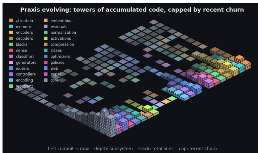
Figure 9: Praxis’s git history as an isometric terrain over the last 2674 commits. Each cell is one subsystem in one time window: a stack of base blocks for its accumulated size (total lines, recency-weighted) topped by a vivid cap for that window’s line churn - the standing codebase carrying the recent activity. Both are weighted by recency (the kernel the model applies to a sequence, turned on the repository): recent windows stack tall with bright caps while history thins toward the always-present prior - the low valley we roll into. Color fades from each subsystem’s hue toward a neutral prior into the past, banded in phased strata over a non-linear timescale. It is the bias/variance geometry read along the frequency axis (see the project notes): loud recent corrections over the quiet, ever-present base. By recency-weighted churn the current center of gravity is core, web, encoders. The framework charts the hand that builds it.
