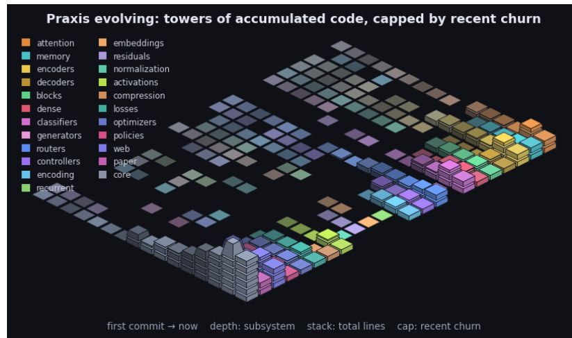
Figure 13: Praxis’s git history as an isometric terrain over the last 2641 commits. Each cell is one subsystem in one time window: a stack of base blocks for its accumulated size (total lines, recency-weighted) topped by a vivid cap for that window’s line churn - the standing codebase carrying the recent activity. Both are weighted by recency (the kernel the model applies to a sequence, turned on the repository): recent windows stack tall with bright caps while history thins toward the always-present prior - the low valley we roll into. Color fades from each subsystem’s hue toward a neutral prior into the past, banded in phased strata over a non-linear timescale. It is the bias/variance geometry read along the frequency axis (see the project notes): loud recent corrections over the quiet, ever-present base. By recency-weighted churn the current center of gravity is core, web, encoders. The framework charts the hand that builds it.
