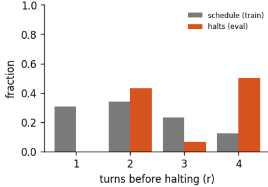
Figure 2: Halting distribution: the fraction of forward passes that stop after r turns, for the 4-turn recurrent loop of run calm-d-1, early-halt rate 19%, mean boundary KL 0.0805. schedule is the random loop-count the model trains under; halts is where the KL gate actually stops at inference. A mass pinned at the maximum (KL never collapsing) is the honest signature of a model that has not yet learned to converge early - the decision is real, not yet decisive.
